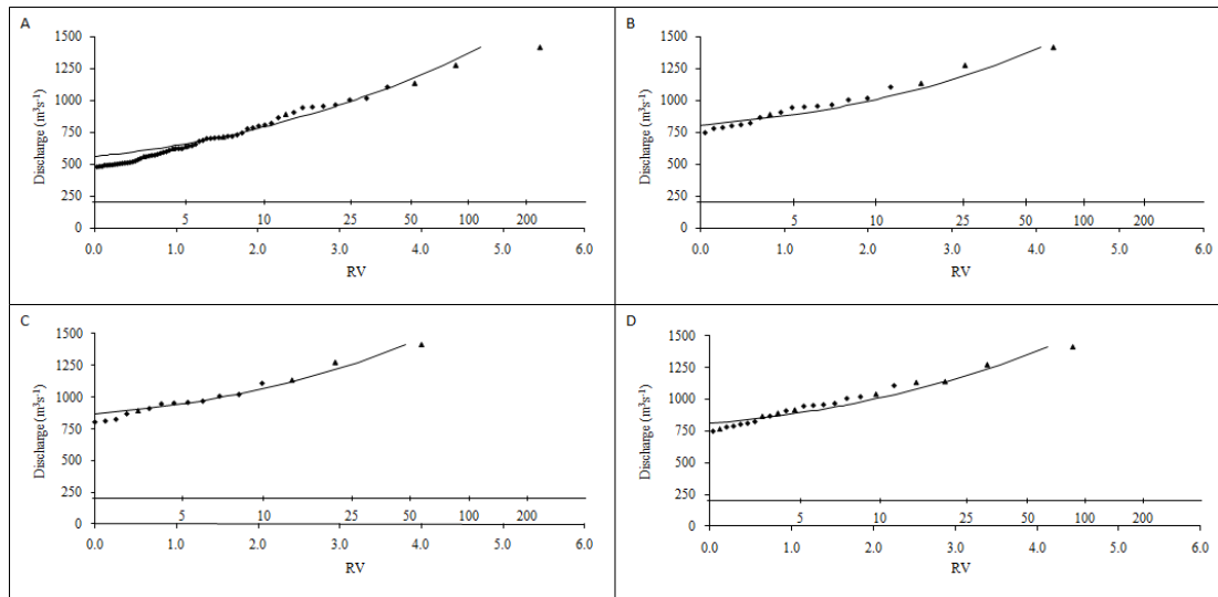
Figure 5 Response of the generalised Pareto distribution based on changes in the threshold (A) represents a threshold of 480 \text{ m}^3\text{s}^{-1} (using the complete augmented record, 1795-2008, but violating the assumption); (B) shows the results if the threshold is set following the criteria to 733 \text{ m}^3\text{s}^{-1} (conforming to the threshold requirements) (1795-2008); (C) illustrates the result of a raised threshold 800 \text{ m}^3\text{s}^{-1} (reduced dataset) (1795-2008); (D) identifies the result on the curve if the complete historical record (1320-2008) is included in the analysis, again using a threshold of 733 \text{ m}^3\text{s}^{-1} .
