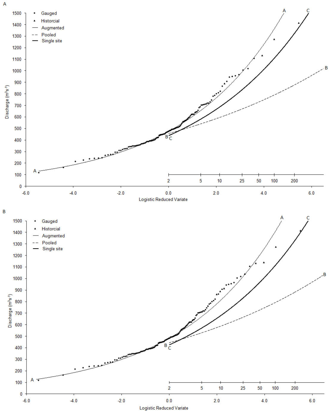
Figure 4 Observed floods from historical and gauged records with curve fitted to combined data set using Bayliss & Reed (2001) method. Results of pooling and single-site analyses (1958–2008) plotted for comparison, relating to return period scale only. (A) 1795–2008 (QMED: 496.3); (B) 1320–2008 (QMED: 514.2). The return period is presented in years.
