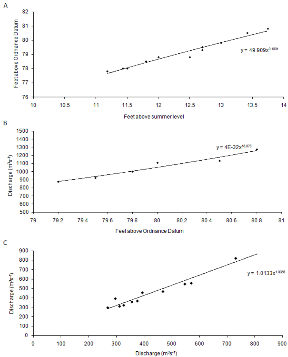
Figure 3 a) Rating curve: comparison of above Ordnance Datum and above summer level (feet) data. b) Rating curve: comparison of feet above Ordnance Datum and discharge ( m^3s^{-1} ) data. c) Rating curve: comparison of the Trent Bridge record from the FSR (IH, 1975) and Colwick gauging station for the overlapping period 1958-1969.
