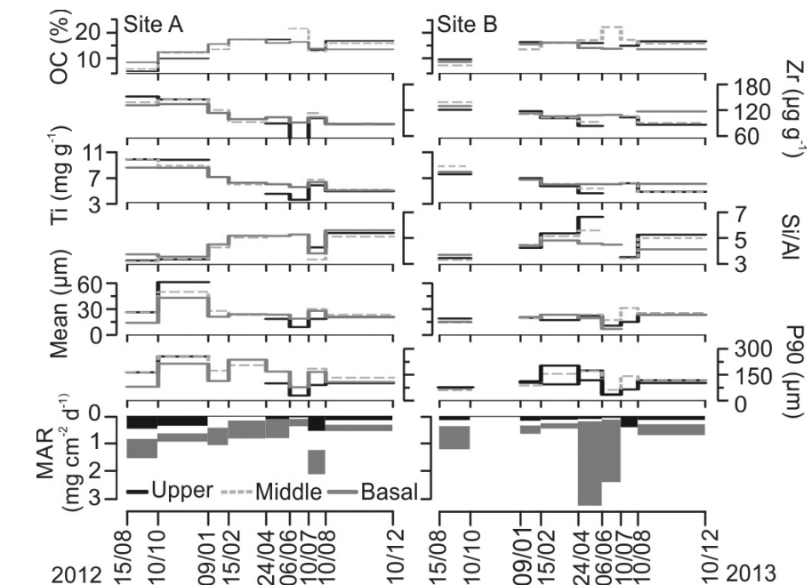
Figure 2. Intra-annual patterns in trapped sediments of organic carbon (OC), Zr, Ti, Si/Al ratio, mean and 90 th percentile grain size, and mass accumulation rate (MAR).
