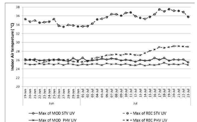
Figure 12: The daily maximum (modelled and recorded) indoor temperatures in the PHV and STV Living rooms
