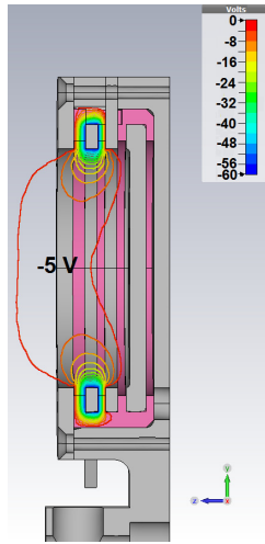
Figure 2: Electrostatic potential distribution for the Prototype 1 Faraday cup biased at -60 V.
