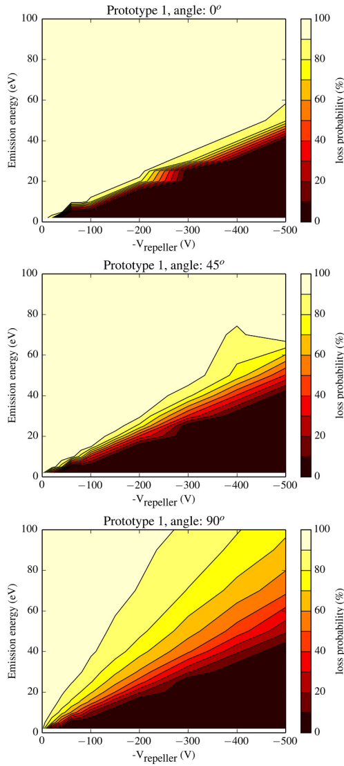
Figure 5: Loss probability of Prototype 1 at different emission energies, repeller ring voltages and maximum emission angle cones of 0°, 45° and 90°.
