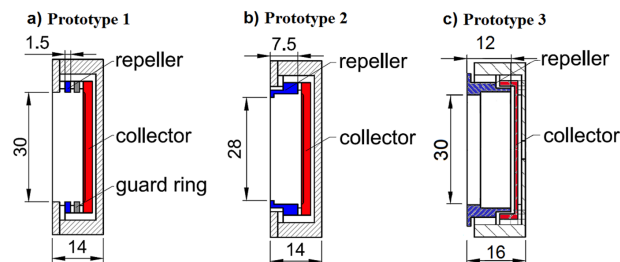
Figure 1: Schematic of the different Faraday cup prototypes developed for HIE-ISOLDE.
