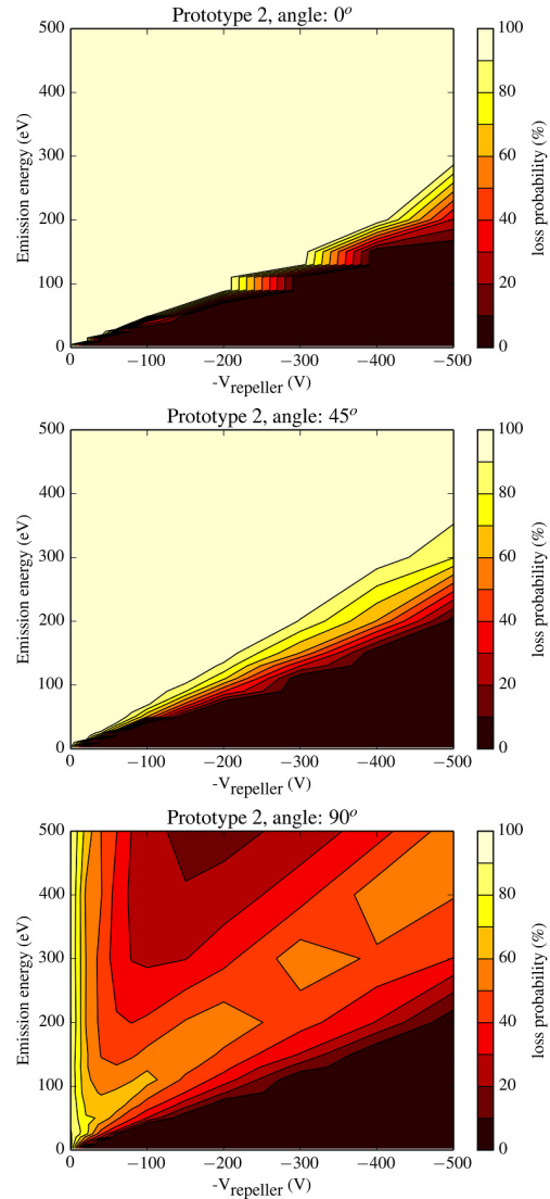
Figure 6: Loss probability of Prototype 2 at different emission energies, repeller ring voltages and maximum emission angles of 0°, 45° and 90°.
