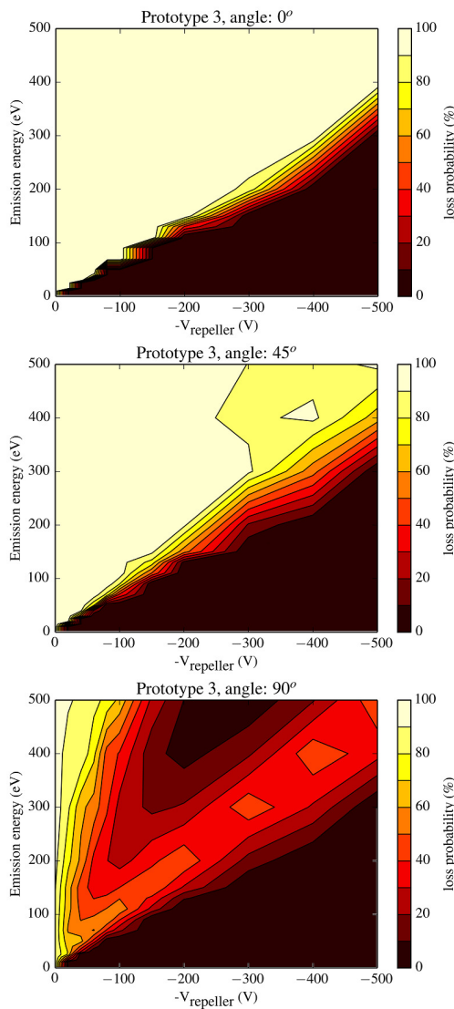
Figure 7: Loss probability of Prototype 3 at different emission energies, repeller ring voltages and maximum emission angles of 0^\circ , 45^\circ and 90^\circ .
