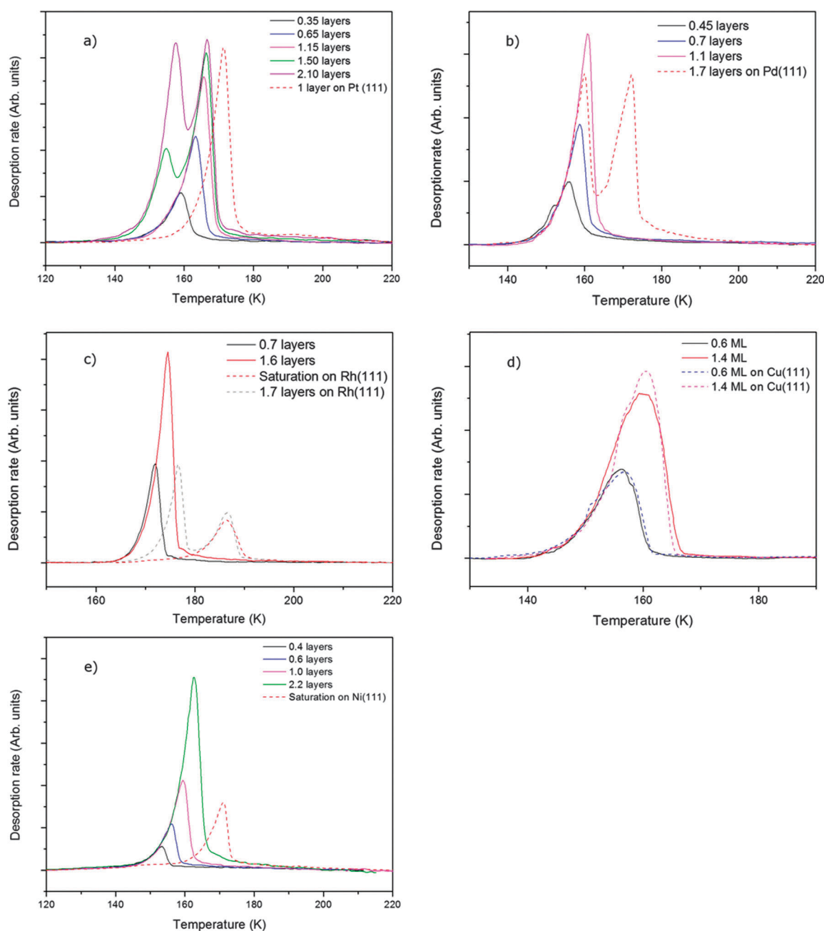
Fig. 2 Temperature programmed desorption of water from (a) SnPt(111), (b) SnPd(111), (c) SnRh(111), (d) SnCu(111), (e) SnNi(111). The coverage of water in the figure legends are with respect to saturation on the relevant clean metal surface, (except Cu, where the number is with respect to an ideal commensurate (\sqrt{3} \times \sqrt{3})R30^\circ structure). The dashed lines show the desorption behaviour of water from the pure metal surface in the absence of the Sn. Water was dosed at ca. 120 K and the heating rates used were 0.8 \text{ K s}^{-1} for SnPt, 0.65 \text{ K s}^{-1} for SnRh and SnPd, 0.5 \text{ K s}^{-1} for SnCu and 0.7 \text{ K s}^{-1} for SnNi.
