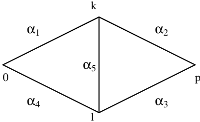
Figure 7: General two loop self energy topology whose value is denoted by \langle \alpha_1, \alpha_2, \alpha_3, \alpha_4, \alpha_5 \rangle .
