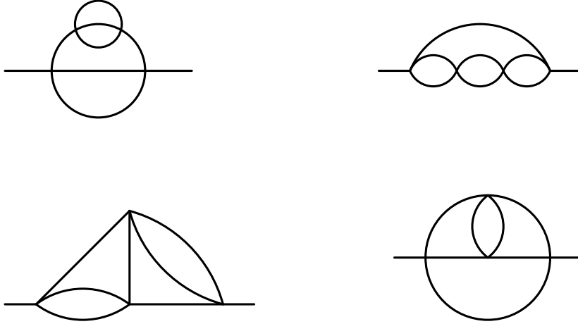
Figure 5: Four loop corrections to the 2-point function.
