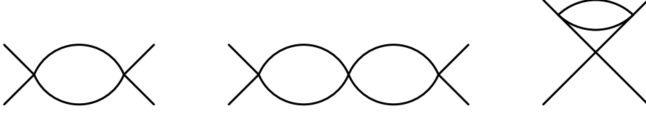
Figure 1: One and two loop corrections to the 4-point function.
