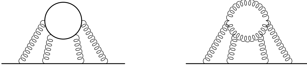
Figure 6: Four loop self-energy corrections in QCD containing d_F^{abcd}d_F^{abcd} and d_F^{abcd}d_A^{abcd} respectively.
