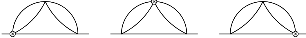
Figure 9: Single evanescent operator correction to the 4 loop 2-point function.
