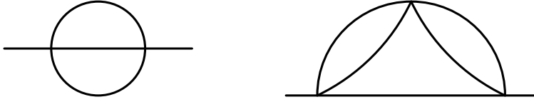
Figure 3: Two and three loop corrections to the 2-point function.
