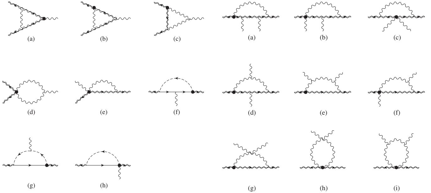
FIG. 1. Diagrams with one gauge, two gaugino lines; the dot represents the position of a C .
