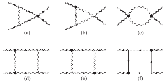
FIG. 3. Diagrams with four gaugino lines; the dot represents the position of a C or |C|^2 .
