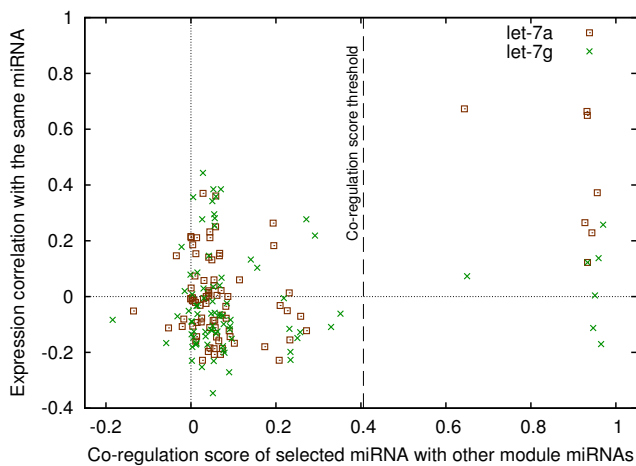
Fig. 3. Co-expression and co-regulation scores between two selected miRNAs and other miRNAs. We call two miRNAs “strongly co-regulating”, if their co-regulation score is above the threshold value. The average co-expression of let-7a with its module member miRNAs is A_{top} = 0.42 . With all miRNAs of the modules this average is A_{all} = 0.027 . Thus, the essentiality of let-7a , relative to other miRNAs, is E = (1 + A_{all}) / (1 + A_{top}) = 0.72 . While let-7a is co-expressed with its strongly co-regulating partners, let-7g is not, and therefore, it is more essential: E = 0.94 .
