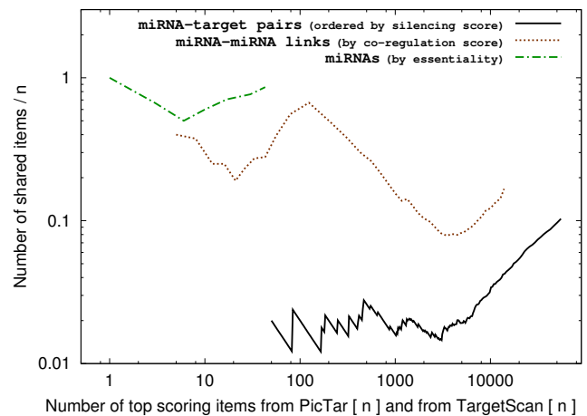
Fig. 5. Comparing TargetScan and PicTar through silencing scores between miRNA - target gene pairs (solid line, this curve is repeated from Fig. 1), miRNA - miRNA co-regulation scores (dotted line) and predicted essentialities of miRNAs (dash-dot). When changing between TargetScan and PicTar as primary data sources the list of top scoring miRNA co-regulation links and the list of predicted most essential miRNAs are clearly much better preserved than the list of top scoring miRNA - target gene pairs. The end points of the two upper curves are higher than the end point of the lower curve, thus, the improvement in data quality cannot be accounted to the reduced number of items ( n ).
