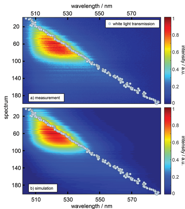
Fig. 3 Comparison of a sequence of measured emission spectra (a) and a sequence of calculated spectra (b) as a function of the resonance wavelength (grey dots) as obtained from the on-axis transmission recorded for the respective resonator setting. The y-axis represents the number of acquired spectra in this series and scales with the stepwise increase of mirror separation. Each spectrum in (b) is composed of the same three Gaussian vibronic bands as in Fig. 2 with relative intensities scaled by the Purcell factor calculated for the respective resonance wavelength and detection function.
