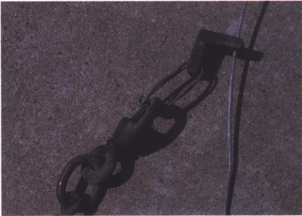
The angled slide wire lock holds the chain at the bottom of the pond.
