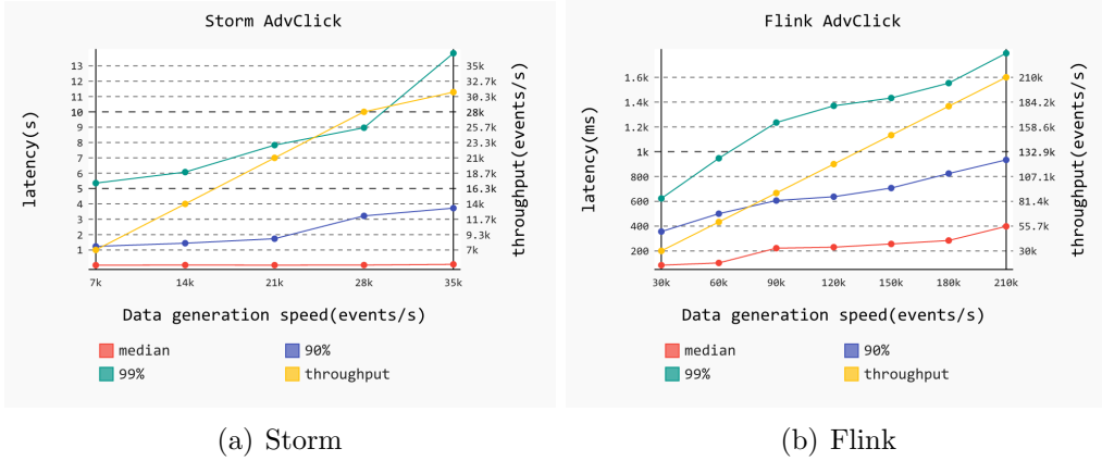
Figure 5.5: AdvClick Performance
