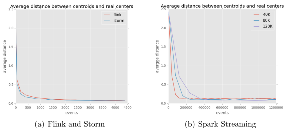
Figure 5.7: Convergences
