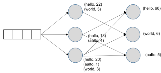
Figure 4.2: Windowed WordCount
