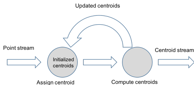
Figure 4.6: Stream k-means scenario
