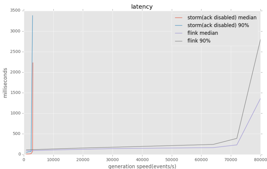
Figure 5.6: KMeans Latency of Flink and Storm
