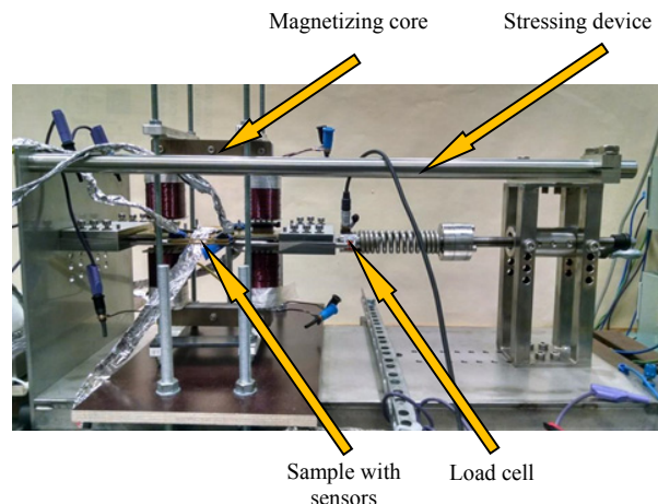
Fig. 1. Experimental setup for measuring unidirectional magnetization curves under stresses parallel to the magnetic field.
