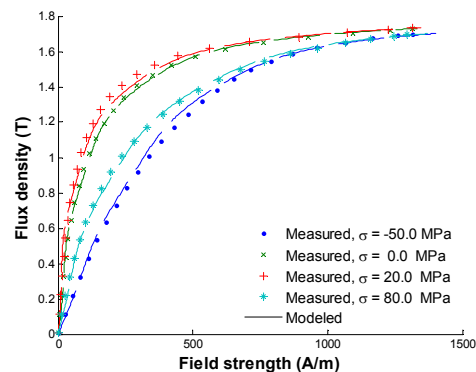
Fig. 2. Fitting the parameters \alpha_i , \beta_i and \gamma_i of the single-valued model to H -averaged B - H curve measurements at different compressive and tensile stresses.
