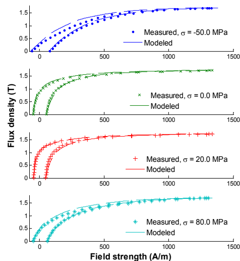
Fig. 3. Fitting the hysteresis model parameters k_0 , a , b , \alpha and c to the B - H curve measurements at different compressive and tensile stresses
