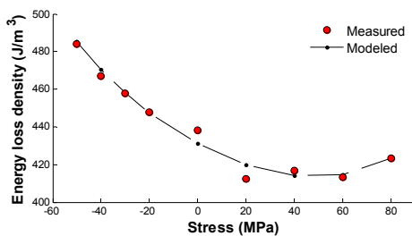
Fig. 4. Comparison of modeled and measured static hysteresis losses at different compressive and tensile stresses.
