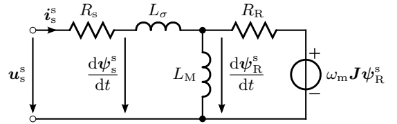
Fig. 1. Inverse- \Gamma model in stator coordinates.
