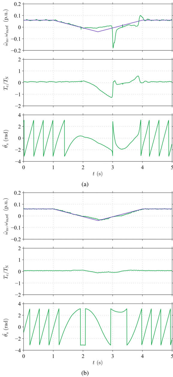
Fig. 8. Experimental results showing no-load speed reversals of the full-order observers: (a) original gains; (b) proposed gains. The first subplot shows the speed reference and the estimated speed, the second subplot shows the estimated torque, and the last subplot shows the estimated rotor-flux angle.
