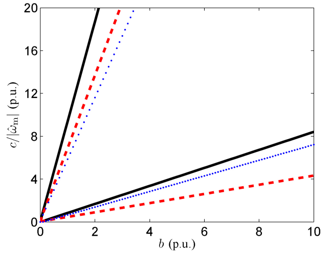
Fig. 3. Areas of stable operation for three different values of i_q for the parameter uncertainties of 10% and \omega_m = 0.05 p.u.: i_q = 0 p.u. (solid line), i_q = 0.8 p.u. (dotted line), and i_q = -0.8 p.u. (dashed line).
