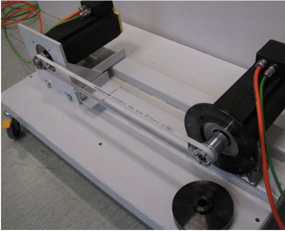
Fig. 2. Experimental setup.
