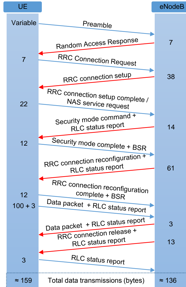
Figure 2. Network access procedure for data transmissions in LTE system.
