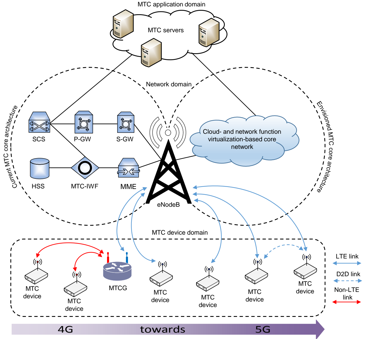
Figure 1. Current and envisioned cellular-based network architectures for supporting MTC services.
