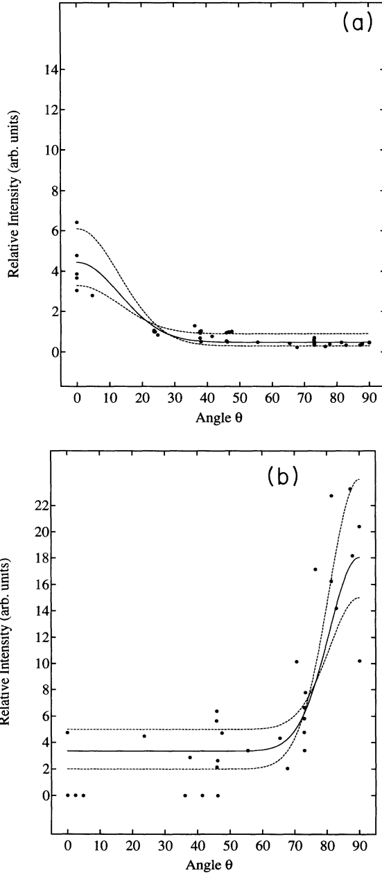
FIG. 4. Distribution of orientation angle \theta (in degrees) for two (\text{Fe}_{0.625}\text{Cu}_{0.375})\text{Sr}_2(\text{Eu}_{1/3}\text{Ce}_{2/3})_3\text{Cu}_2\text{O}_{11} specimens oriented (a) with the magnetic field perpendicular to the sample surface and (b) with the magnetic field parallel with the surface. The distributions were obtained from x-ray diffraction spectra.
