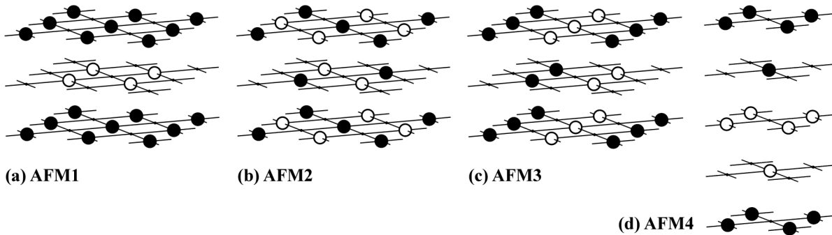
FIG. 2. Schematic of the four AFM orderings used in calculating the magnetic exchange constants of \text{Sr}_2\text{Cu}(\text{W},\text{Mo})\text{O}_6 . Black spheres correspond to Cu ions with spin up, and white spheres to Cu ions with spin down. Other ions and the long bonds along c axis are omitted from view for clarity.
