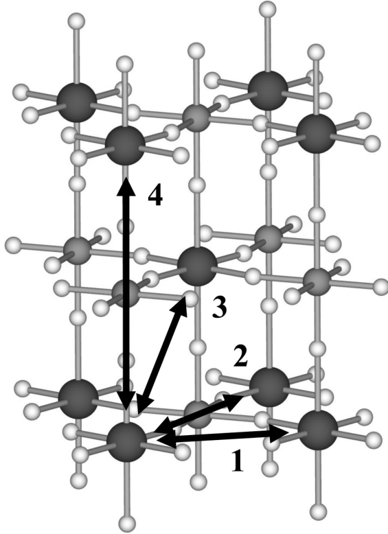
FIG. 1. Schematic of the exchange constants J_1 - J_4 between Cu ions in the \text{Sr}_2\text{Cu}(\text{W},\text{Mo})\text{O}_6 double perovskites. Large dark-gray spheres are Cu, smaller light-gray spheres are W/Mo, and small white spheres are O. Sr is omitted from view for clarity.
