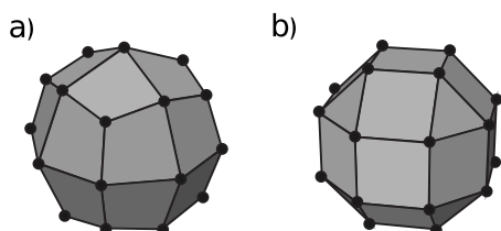
FIG. 2. Polyhedra used in atomic meshes of (a) deltoidal icositetrahedron and (b) rhombicuboctahedron.
