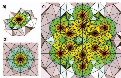
FIG. 4. Cut plane of the molecular mesh of the C_6H_6 molecule with parameters q = \sqrt{2} , s \geq \sqrt{1/3} , and 15 outer layers (see text): (a) the complete mesh (diameter of 55 Å), (b) the atomic mesh near a carbon nucleus, and (c) the close-up of the molecular region.
