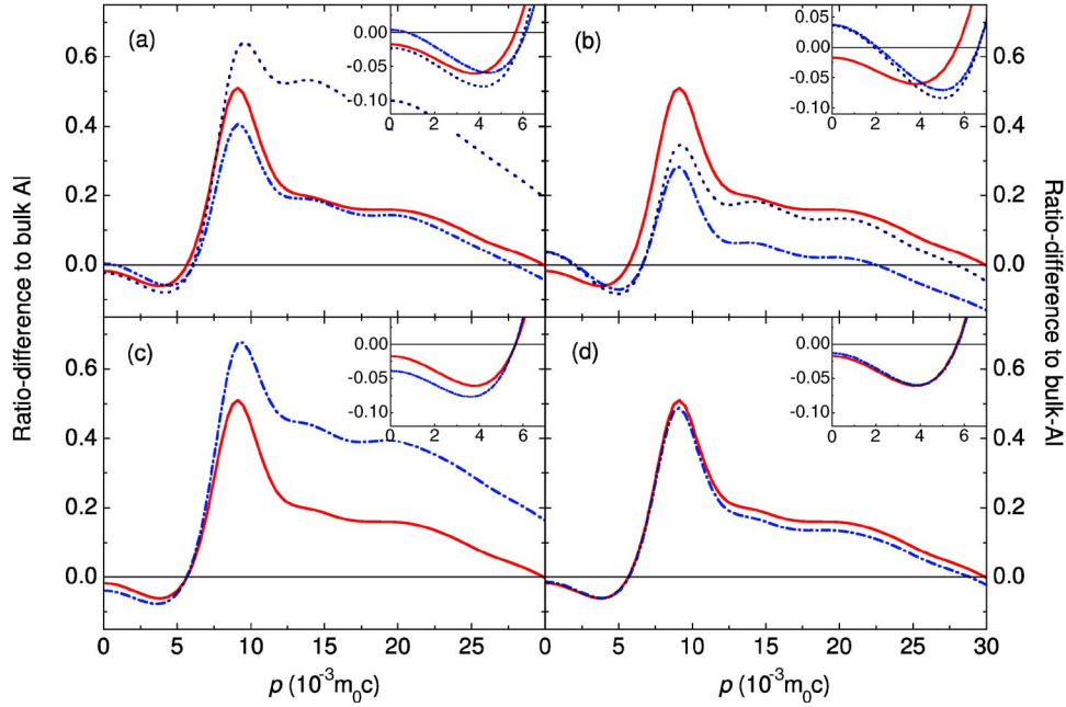
FIG. 3. (Color online) Influence of different approximations on the first-principles results for Al vacancies decorated with Cu atoms. In all panels, the solid (red) line shows the RD spectrum obtained for the Al vacancy surrounded by three Cu atoms on the [100] plane in the strained Al lattice including ionic relaxation due to the electronic structure and the localized positron state. (a) The dash-dotted (dark blue) and the dotted (blue) lines show the results corresponding to ideal (no relaxation) ion positions and for two and three Cu atoms, respectively. (b) The dash-dotted (dark blue) and the dotted (blue) lines correspond to the Al lattice without strain and to three and four Cu atoms, respectively. (c) The dash-dotted (dark blue) curve shows the result for three Cu atoms nearest neighbors to each other. (d) The dash-dotted (dark blue) curve corresponds to the fit using the linear combination of RD spectra for two and four Cu atoms with equal weights.
