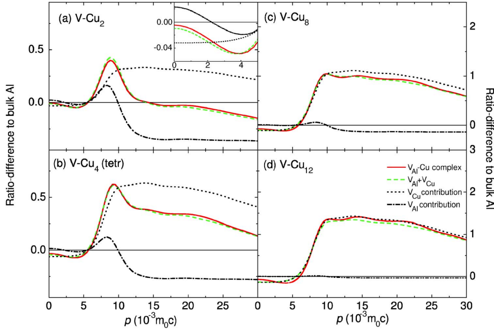
FIG. 4. (Color online) CDB RD spectra for vacancy-Cu complexes in Al-Cu alloys with (a) 2, (b) 4, (c) 8, and (d) 12 nearest neighbor Cu atoms. The tetragonal configuration is used in the case of four Cu atoms. The solid (red) curves give the results of the first-principles calculations. The dashed (green) curves are the linear combinations [Eq. (2)] of the RD spectra calculated for vacancies in strained Al and Cu. The dash-dotted and dotted curves show the Al and Cu contributions, respectively. The inset in (a) shows the magnified low-momentum region.
