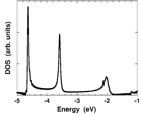
FIG. 4. Projected density of the m=0 symmetry states as function of the energy. The WPP results are shown for the nanos island comprising 19 Na atoms. The energy is referred to the vacuum level.
