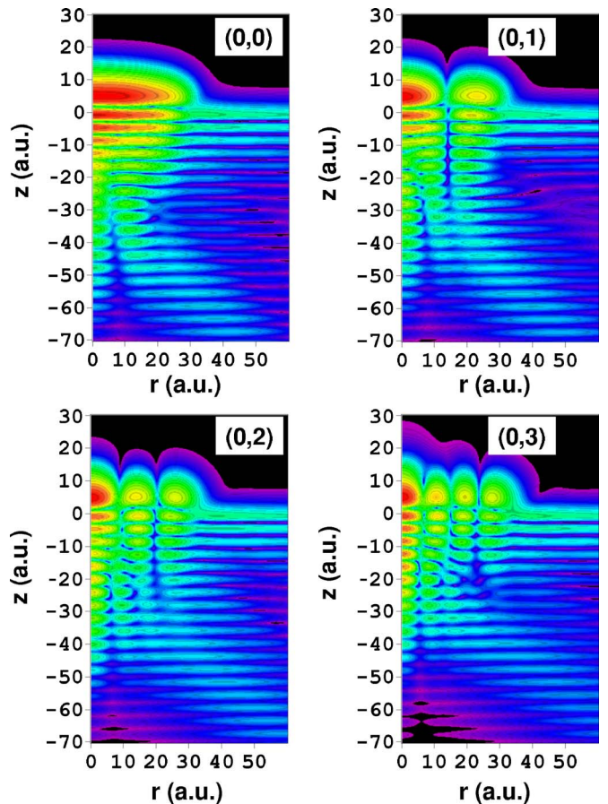
FIG. 5. (Color online) Interpolated images of the electron density of the (m=0, n=0, 1, 2, 3) quasistationary island-localized states for the 61 Na atom island on the Cu(111) surface. The logarithm of the density \ln\{|\psi_m^{res}(r, z, E_{mn})|^2\} is shown in cylindrical coordinates, parallel ( r ) and perpendicular ( z ) to the surface. z=0 corresponds to the position of the image plane of the Cu(111) surface (Ref. 37), and inside the metal z is negative. The electron density decreases from 1 to 0.001 (arbitrary units) when going from red to violet. The states are labeled according to their quantum numbers, as explained in the text.
