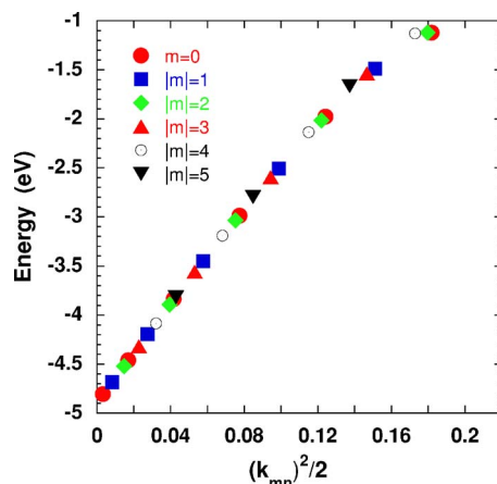
FIG. 8. (Color online) Energy of various (m, n) quasistationary states of 61 Na atom nanoisland on Cu(111). The energy is referred to the vacuum level. The results are shown as a function of the quantized wave vector of the corresponding particle-in-a-box states (see the text for the definition). The different symbols represent states of the different m symmetries, as shown in the inset.
