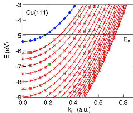
FIG. 3. (Color online) Electronic structure of the clean Cu(111) surface system according to our DFT calculations. The filled circles and stars denote m=0 energy eigenvalues and correspond to the surface and bulk states, respectively. Few m=1 eigenvalues are given by open green squares. The identification of the parallel momentum values is explained in the text. The solid lines correspond to the parabolic free-electron dispersion with unit effective mass. The thick red lines bracket the projected bulk bands and the blue line is the surface state band. The black horizontal line denotes the Fermi level.
