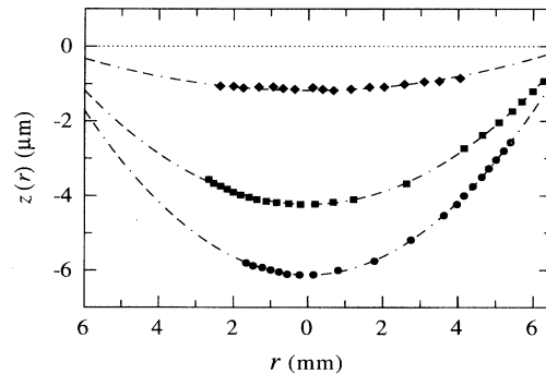
FIG. 3. Surface profiles from a “rapid stopping experiment,” performed on a d = 0.4 mm thick layer of ^3\text{He-B} at T = 0.76T_c ; r is the distance from the rotation axis. From bottom to top: snapshots at the speed \Omega = 1.55 rad/s, at t = 0.2 s, and t = 0.8 s after deceleration was started. The dotted line represents the horizontal free surface and the dash-dotted curves depict paraboloids fitted to the experimental points.
