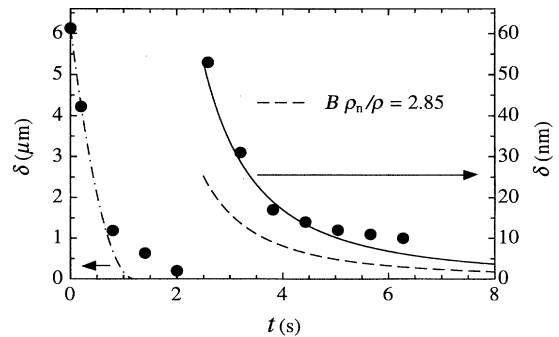
FIG. 4. Relaxation of the nadir in the \Omega -induced parabola as a function of time during and after deceleration of the ^3\text{He-B} sample from the equilibrium vortex state at \Omega = 1.55 rad/s. Corresponding surface profiles for the first three data points are given in Fig. 3. Note that the right hand scale is magnified by 100 \times . The dash-dotted curve represents \delta for the instantaneous speed of the cryostat during linear deceleration; for explanations of the other curves, see text.
