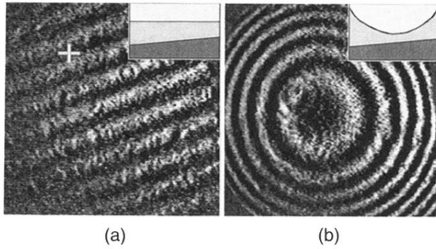
FIG. 1. Interferograms (20 ms long “snapshots”) of (a) non-rotating and (b) rotating ( \Omega = 1.55 \text{ rad/s} ) samples of ^3\text{He-B} . The adjacent fringes correspond to a change of 0.310 \mu\text{m} in liquid thickness above the tilted reference glass as is illustrated in the insets. The white cross in (a) defines the center of the optical cell. The displayed area of the interferograms is 5 \times 5 \text{ mm}^2 .
