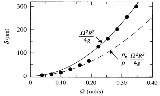
FIG. 2. Absolute change \delta of the liquid height in the center of the \Omega -induced parabola during acceleration as compared with the stationary free surface level for a 0.1 mm thick layer of ^3\text{He-B} . The solid and dashed curves mark the calculated behavior for a classical liquid and for a vortex-free superfluid with a flattened meniscus at T = 0.68T_c , respectively. Note the transition from the vortex-free behavior ( \mathbf{v}_n = \Omega \times \mathbf{r} , \mathbf{v}_s = 0 ) to the “classical” curve \mathbf{v}_n = \mathbf{v}_s = \Omega \times \mathbf{r} at \Omega \approx 0.20 rad/s. The size of the data points is approximately equal to the experimental error bars.
