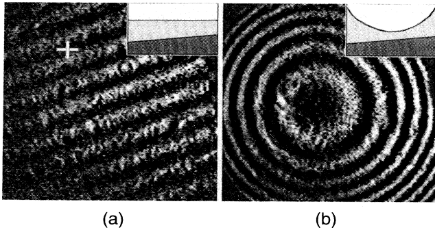
FIG. 1. Interferograms (20 ms long “snapshots”) of (a) non-rotating and (b) rotating ( \Omega = 1.55 rad/s) samples of ^3\text{He-B} . The adjacent fringes correspond to a change of 0.310 \mu\text{m} in liquid thickness above the tilted reference glass as is illustrated in the insets. The white cross in (a) defines the center of the optical cell. The displayed area of the interferograms in 5 \times 5 \text{ mm}^2 .
