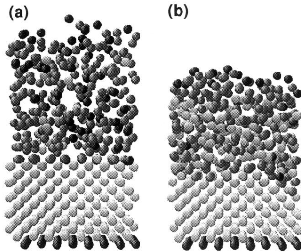
FIG. 3. Snapshots of the two films grown with (a) E_{\text{beam}} = 1 and (b) E_{\text{beam}} = 40 eV after growth and relaxation of 7 ps. The black, grey, and white spheres correspond to twofold-, threefold-, and fourfold-coordinated atoms, respectively. The total number of atoms is N = 678 (a) and N = 674 (b).
