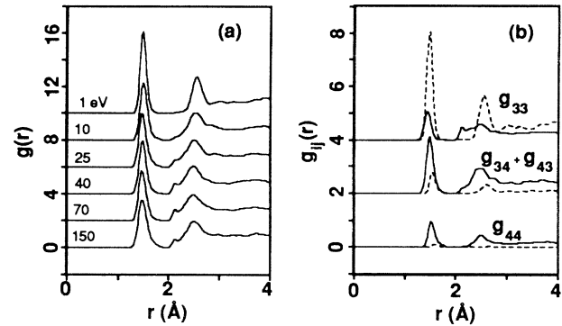
FIG. 2. (a) Pair correlation function g(r) for the films grown with E_{\text{beam}} = 1, 10, 25, 40, and 70 eV and the film obtained by shooting 125 particles with energy E_{\text{beam}} = 150 eV on the 40-eV film. Note the emergence of the shoulder in the second-neighbor peak with increasing beam energy. (b) Pair correlation function g_{ij}(r) of atoms with coordination numbers (i, j) = 3, 4 for the films grown with E_{\text{beam}} = 1 and 40 eV. The dashed and solid lines correspond to the 1- and 40-eV films, respectively. Note the peak in g_{33}(r) for E_{\text{beam}} = 40 eV. g(r) = \sum_i g_{ii}(r) + \sum_{i \neq j} g_{ij}(r) .
