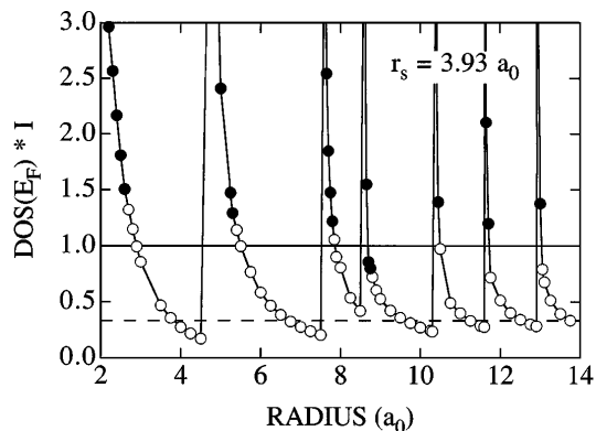
FIG. 3. Na jellium wires with r_s = 3.93a_0 . The Stoner criterion product I\tilde{D} is given as a function of the radius of the wire. The regions of stable magnetic and spin-compensated solutions are marked by black and open circles, respectively. The product for the infinite jellium with r_s = 3.93a_0 is given for comparison (dashed line).
