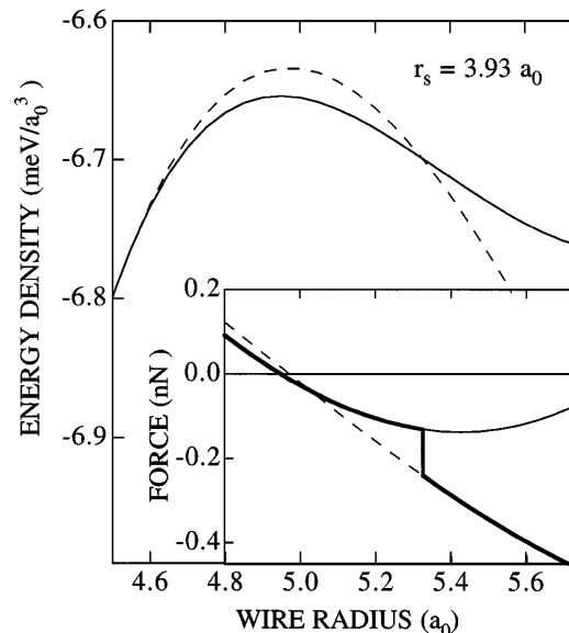
FIG. 4. Na jellium wires with r_s = 3.93a_0 . The total energy per volume as a function of the wire radius. The second subband is occupied when the radius is larger than \sim 4.7a_0 . The energies when the second subband is fully spin polarized (solid line) and spin compensated (dashed line) are shown. The ensuing elongation forces are given in the inset. The thick line gives the adiabatic behavior of the force when the wire narrows.
