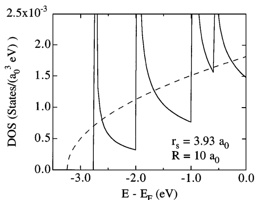
FIG. 2. Na jellium wire with r_s = 3.93a_0 and a radius of 10a_0 . The density of states (DOS) per unit volume is given as a function of the energy. The position of the Fermi energy defines the energy zero. The DOS for the infinite jellium with r_s = 3.93a_0 is given for comparison (dashed line).
