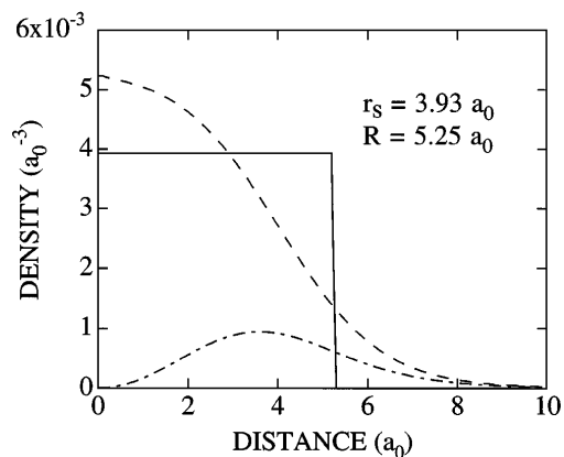
FIG. 1. Na jellium wire with r_s = 3.93a_0 and a radius of 5.25a_0 . The total electron density n_{\uparrow}^{\downarrow}(r) + n_{\downarrow}^{\uparrow}(r) (dashed line), the spin density n_{\uparrow}^{\downarrow}(r) - n_{\downarrow}^{\uparrow}(r) (dash-dotted line), and the positive background charge n_+ (solid line) are given as a function of the distance from the cylinder axis.
