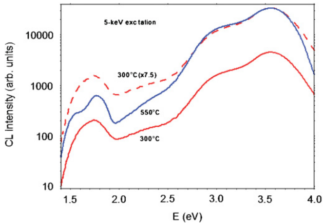
FIG. 3. (Color online) Cathodoluminescence spectra for Ga-doped ZnO samples grown at 200 °C in pure Ar and annealed at 300 and 550 °C, respectively, in forming gas. The dashed curve represents the 300 °C sample intensity normalized to that of the 550 °C sample in the near-band-edge region (3.5 eV) in order to compare the relative intensities of the peaks near 1.8 eV.
