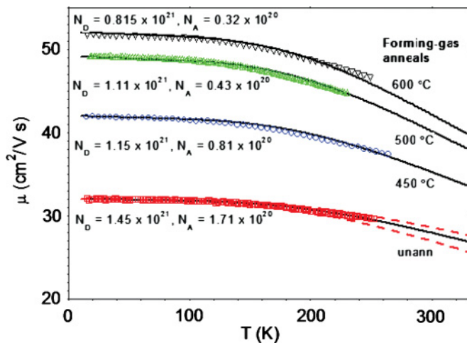
FIG. 1. (Color online) Experimental (points) and theoretical (solid and dashed lines) mobilities for Ga-doped ZnO samples grown at 200 °C in pure Ar and annealed at various temperatures in forming gas.
