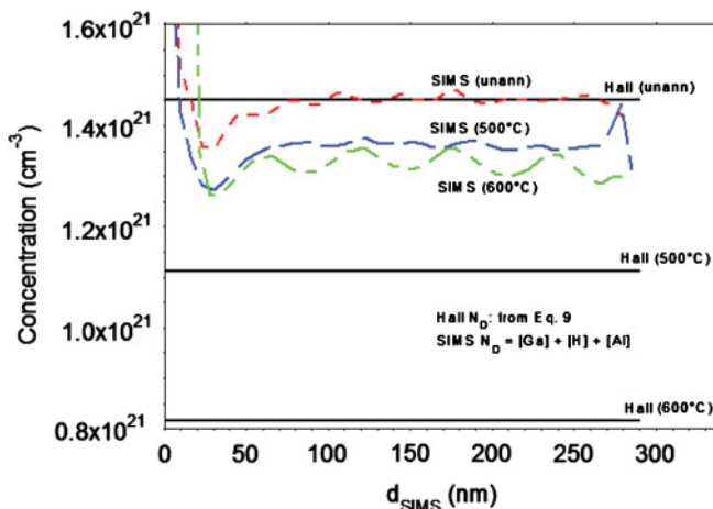
FIG. 2. (Color online) A comparison of donor concentrations determined by Hall mobility analysis (solid lines) and SIMS measurements of [Ga] + [H] + [Al] (dashed lines).
