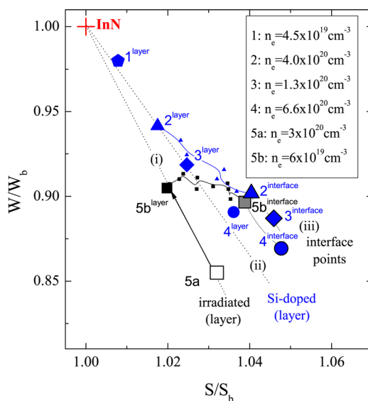
FIG. 3. (Color online) SW plot of the measured line-shape parameters representative for the near-surface (“layer,” filled symbols) and near-interface (“interface,” black border) areas of the InN samples. Different symbols are used for different samples. Si-doped samples are depicted in blue (light color) and irradiated in black (dark color). All parameters are normalized by a suitable reference for the InN lattice.
