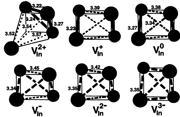
FIG. 2. The nearest-neighbor relaxations around In vacancies. The bond lengths are in Å.
