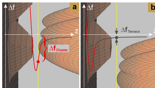
FIG. 7. (Color online) Drawing explaining the contrast formation in the constant height mode imaging of nanoclusters. The tip, which was used for the calculations, keeps a pathway with a constant height above the surface (yellow dotted line). (a) If the tip is above the cluster, it is only the last nanometer of the tip which is placed in the short-range interaction between tip and cluster, producing a large cluster contrast \Delta f_{\text{cluster}} . (b) As soon as the tip has passed the cluster, the tip is at a distance of the cluster height far away from the surface. The detuning value \Delta f_{\text{terrace}} is then very small.
