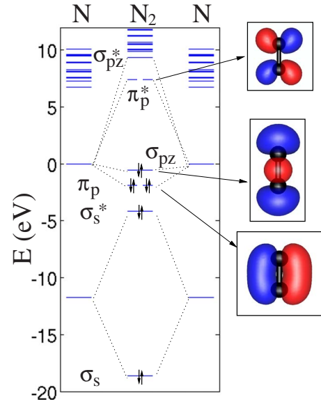
FIG. 7. (Color online) (Left) Energy level diagrams for individual N atoms and the N_2 molecule as calculated with VASP. N_2 energy levels are interpreted using the molecular-orbital theory. The net spin polarization of the N_2 molecule is zero, so including the electron spin in the calculations does not affect the results. Some one-electron states (from a SIESTA calculation) have been included in the insets: color red (blue) corresponds to positive (negative) values of the wave function.
