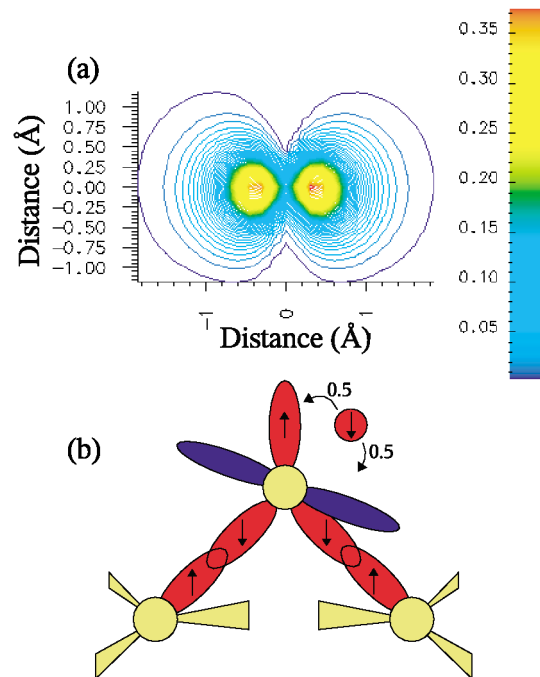
FIG. 2 (color). (a) The spin density in e/\text{\AA}^3 of a plane normal to the surface through the center of the adatom when the adatom is at the equilibrium position. The adatom is at (0,0). (b) A schematic diagram of the bond orbitals at the equilibrium position in a plane through the adatom and the two surface carbons. Note that this schematic is a projection, and that the blue p orbital is orthogonal to the adatom-surface bonds.
