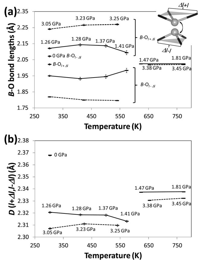
FIG. 7. (a) B -cation (Zr or Ti) and oxygen bond lengths in the rhombohedral phase. The difference between B-O_{\Delta l+} and B-O_{\Delta l-} bond lengths increases with increasing pressure. The decrease in difference seen at 1.41 GPa pressure is probably related to the vicinity of the transition to the cubic phase. (b) The distance D(l + \Delta l, l - \Delta l) between the oxygen triangles. In both panels, the 3 GPa data are indicated by dotted lines. The inset shows the displacement of the B cations under pressure. At ambient pressures, the B is closer to the larger triangle and displaces towards smaller triangle under pressure.
