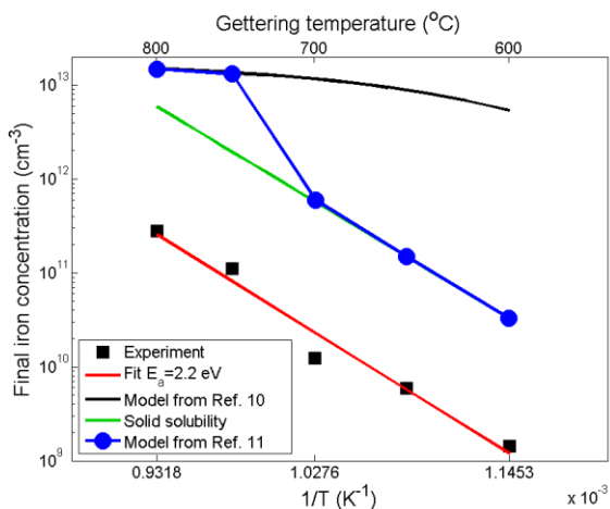
Figure 1 Measured iron concentration in the bulk (black squares) after low-temperature anneals and fitted Arrhenius relation with an activation energy of 2.2 eV (red line). Black line represents iron concentrations calculated by using the solubility model [10] and blue spheres represent iron concentrations calculated by using the model including both segregation and precipitation [11].
