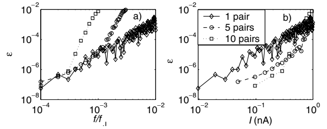
FIG. 3. Error (a) in the pumped charge over a single period and (b) in the current as a function of (a) frequency and (b) current. Here C_J = C , C_g = 0.1C , E_J^{\text{max}} = e^2/C , and f_J = E_J^{\text{max}}/\hbar . The error is \epsilon \equiv 1 - Q_p/2ne \equiv \Delta I/I . The line marked by diamonds represents pumping a single Cooper pair, the line marked by circles represents pumping five Cooper pairs, whereas the squared line represents pumping ten Cooper pairs per cycle. In (b) we assume f_J = 300 \times 10^9 \text{ s}^{-1} .
