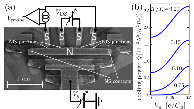
FIG. 1 (color online). (a) Scanning electron micrograph of the heat transistor, showing also the measurement setup. In the middle, the normal-metal (Cu) island subjected to cooling. Four superconducting probes (Al) with Al-Ox tunnel junctions can be seen above, and truncated capacitor plates (Al) with direct NS contacts on the left and right. (b) Theoretical heat flow from the N island at the optimal bias point at different temperatures as a function of the gate voltage. T denotes the common temperature of the island electrons and quasiparticles in the superconductor, and T_c = \Delta/(1.764k_B) is the superconducting critical temperature.
