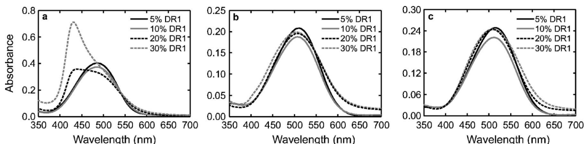
FIG. 2. Absorption spectra of thin films of (a) DR1 in PS, (b) DR1 in PVPPh, and (c) DR1 in P4VP.
