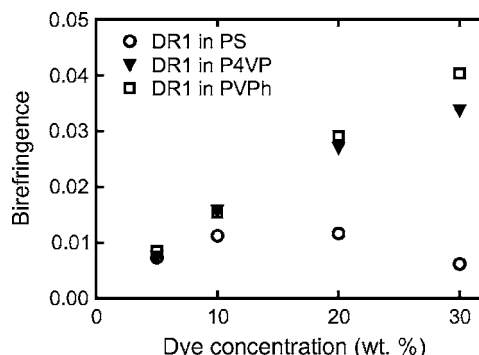
FIG. 3. Photoinduced birefringence as a function of dye concentration for DR1 in PS, P4VP, and PVPPh. The reported values are the saturation values of the birefringence while the writing beam is applied on the sample. The writing beam intensity was 150 mW/cm 2 .
