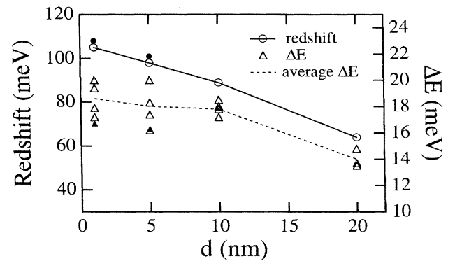
FIG. 5. Experimental redshift ( \circ ) and peak splitting \Delta E ( \triangle ) of adjacent peaks as a function of d . The lines are guide to an eye. The calculated values for the redshift and \Delta E , shown by respective filled symbols, are close to the experimental values for d=1 and 5 nm.
