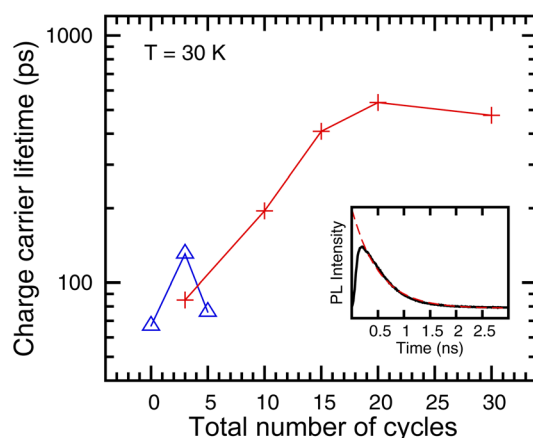
FIG. 3. Charge carrier lifetimes as a function of the cycles of AlN (+) and ammonia plasma ( \Delta ) deposited at 150 °C. The inset shows a typical exponential fit to the measured data.
