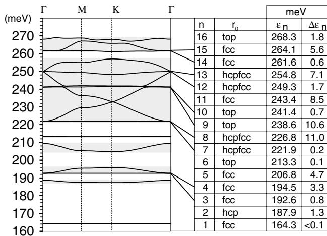
FIG. 4. The lowest vibrational branches for H/Pt(111). \epsilon_n denotes the band center, \Delta\epsilon_n the bandwidth, and r_0 the center of the BS with \vec{k} = 0 .
