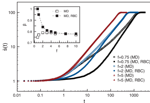
FIG. 13. The translocation coordinate \bar{s} as a function of time from MD simulations. The chain is either allowed to escape the pore to the cis side (open symbols, same data as in Fig. 10) or such an escape is prevented by a reflecting boundary condition (RBC, filled symbols). The results change drastically, if the RBC is used. Inset: the scaling exponent \beta ( \langle \bar{s}(t) \rangle \sim t^\beta ) as a function of the driving force f both without and with the RBC. Parameters are the same as in Fig. 10.
