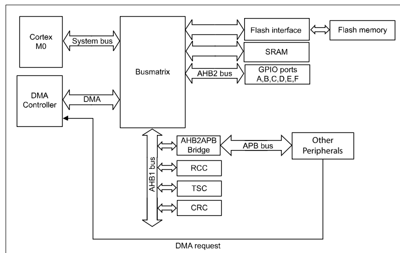
Figure 1. General STM32F0 Architecture
