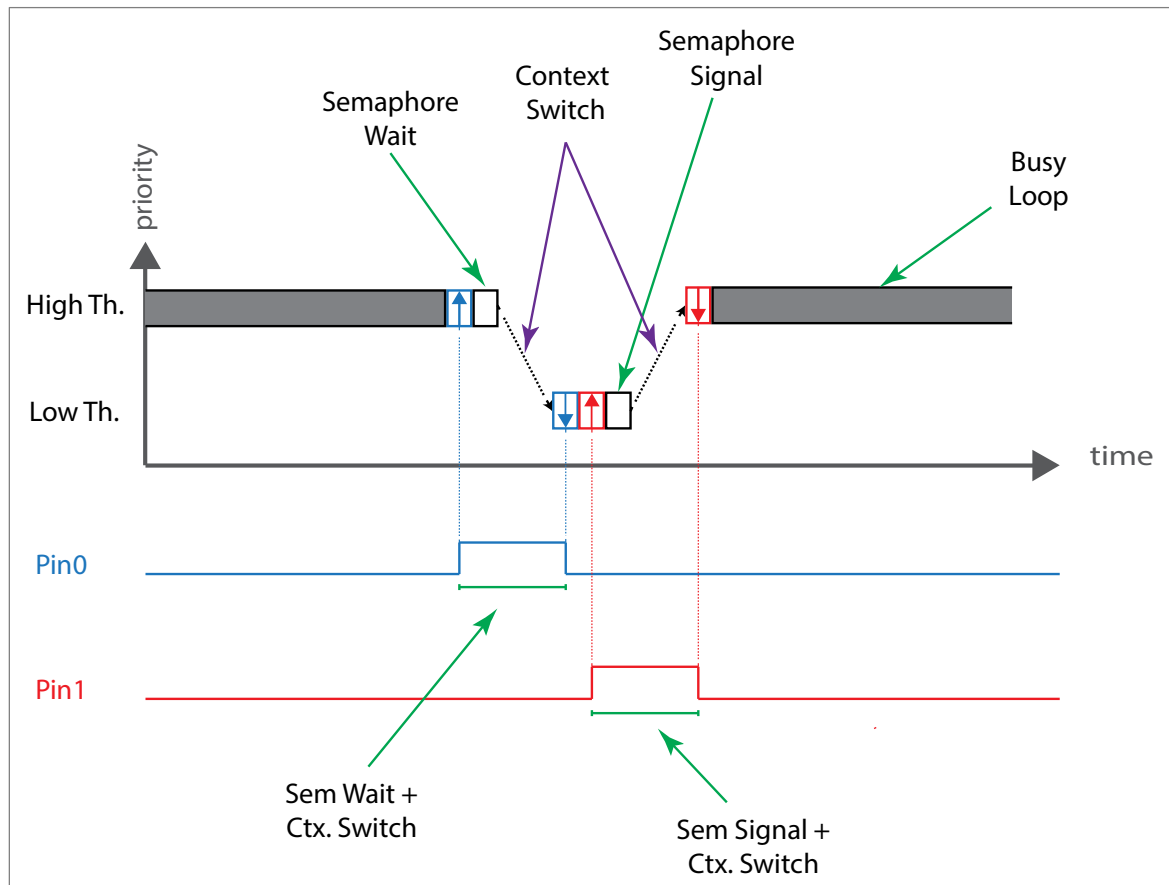
Figure 14. Detail of Context Switch
