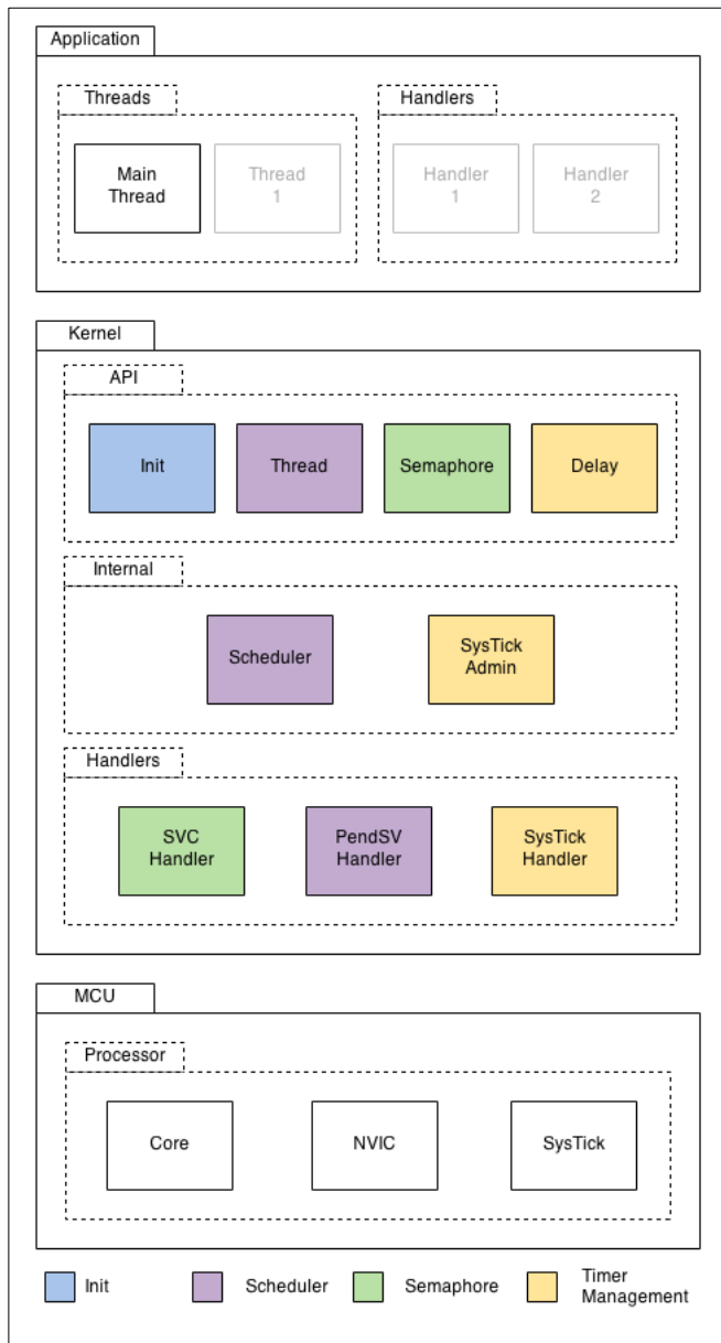
Figure 3. General Architecture
