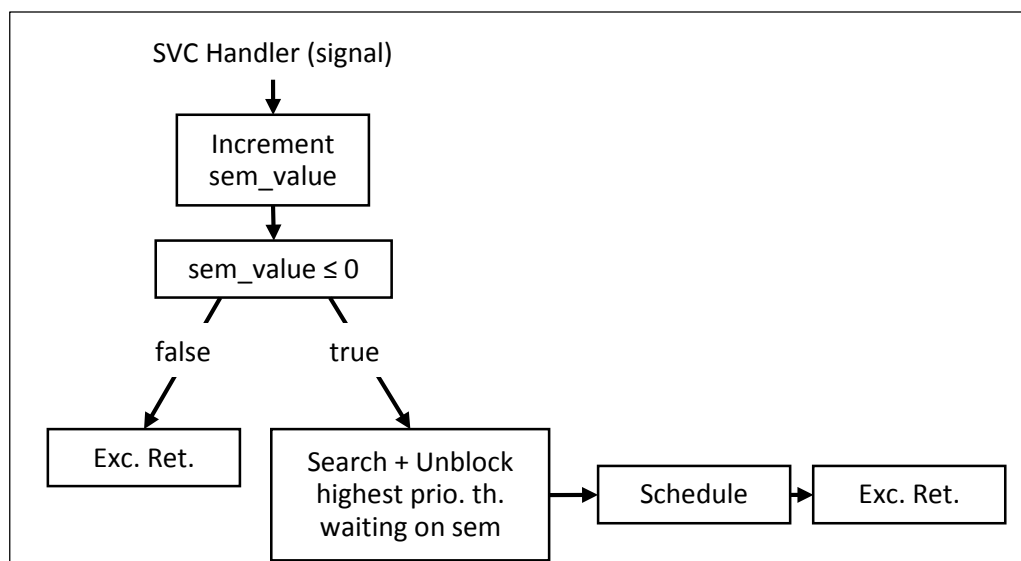
Figure 10. Semaphore Signal Operation
