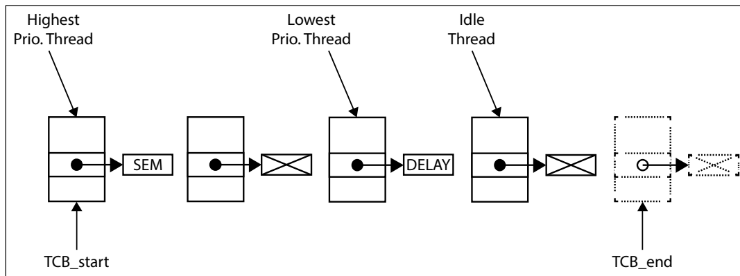
Figure 5. TCB array example for 3 user threads + idle thread
