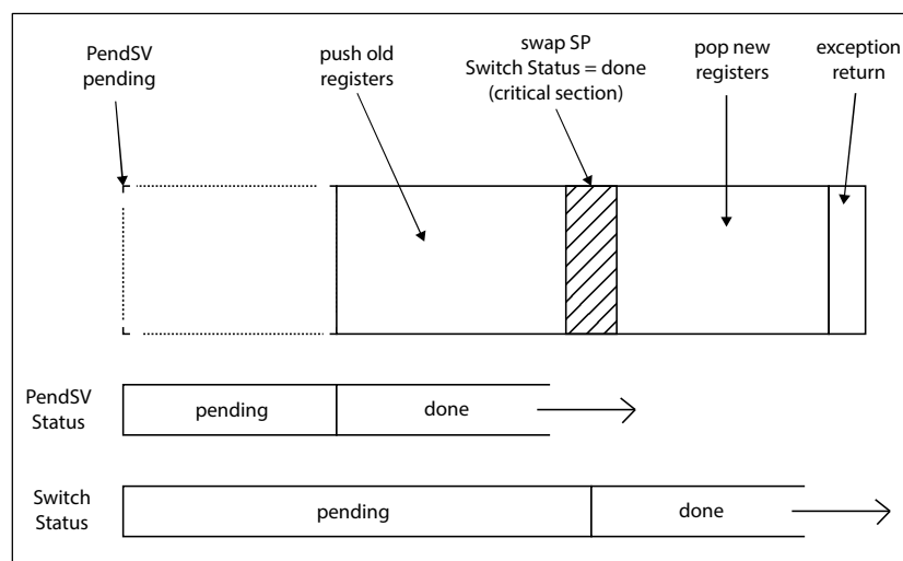
Figure 8. PendSV normal progress, with status of flags
