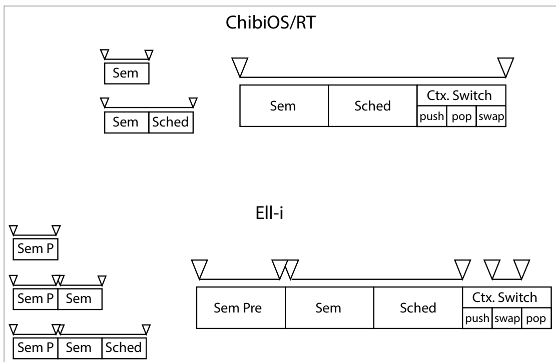
Figure 15. Blocking Time Diagram for Wait Operation for ChibiOS and ELL-i
