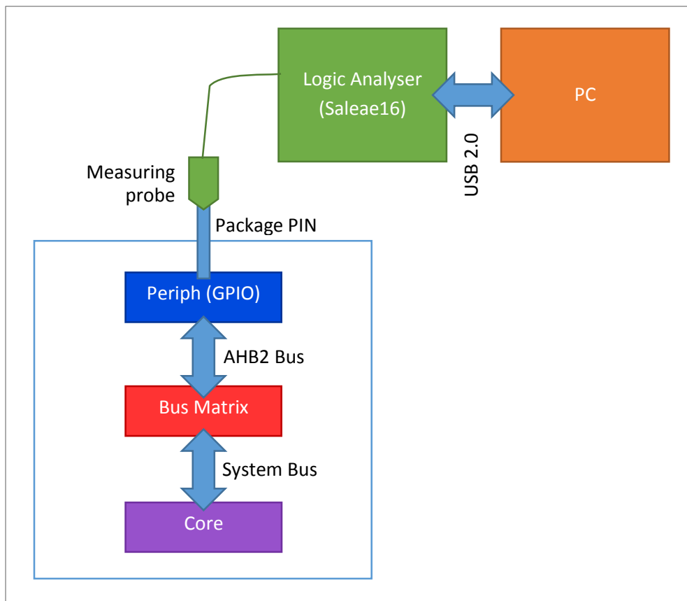
Figure 13. Hardware Testing Framework
