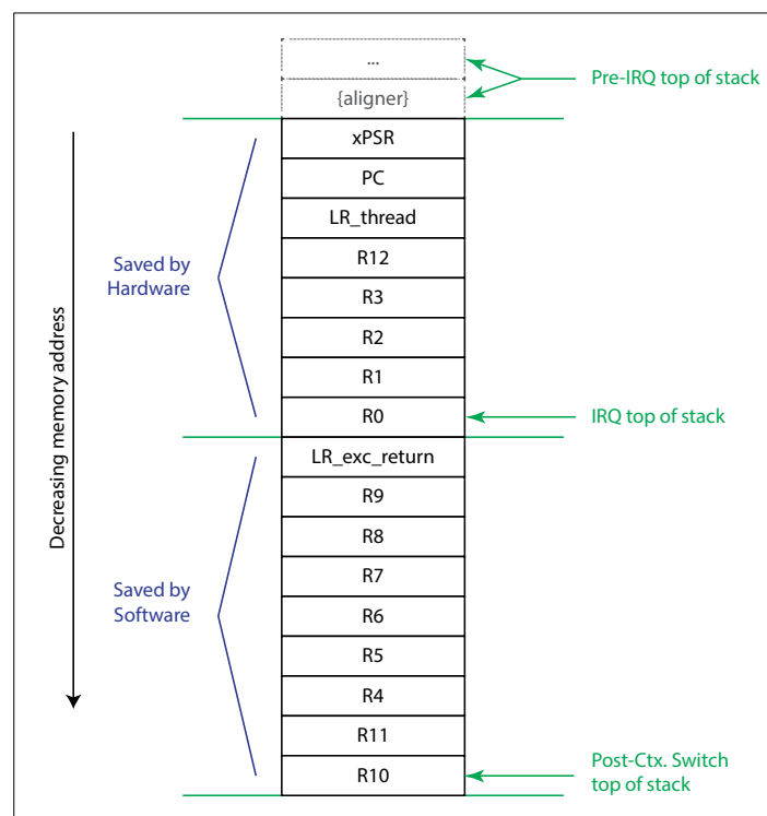
Figure 2. Context Switch Prototype Context Frame
