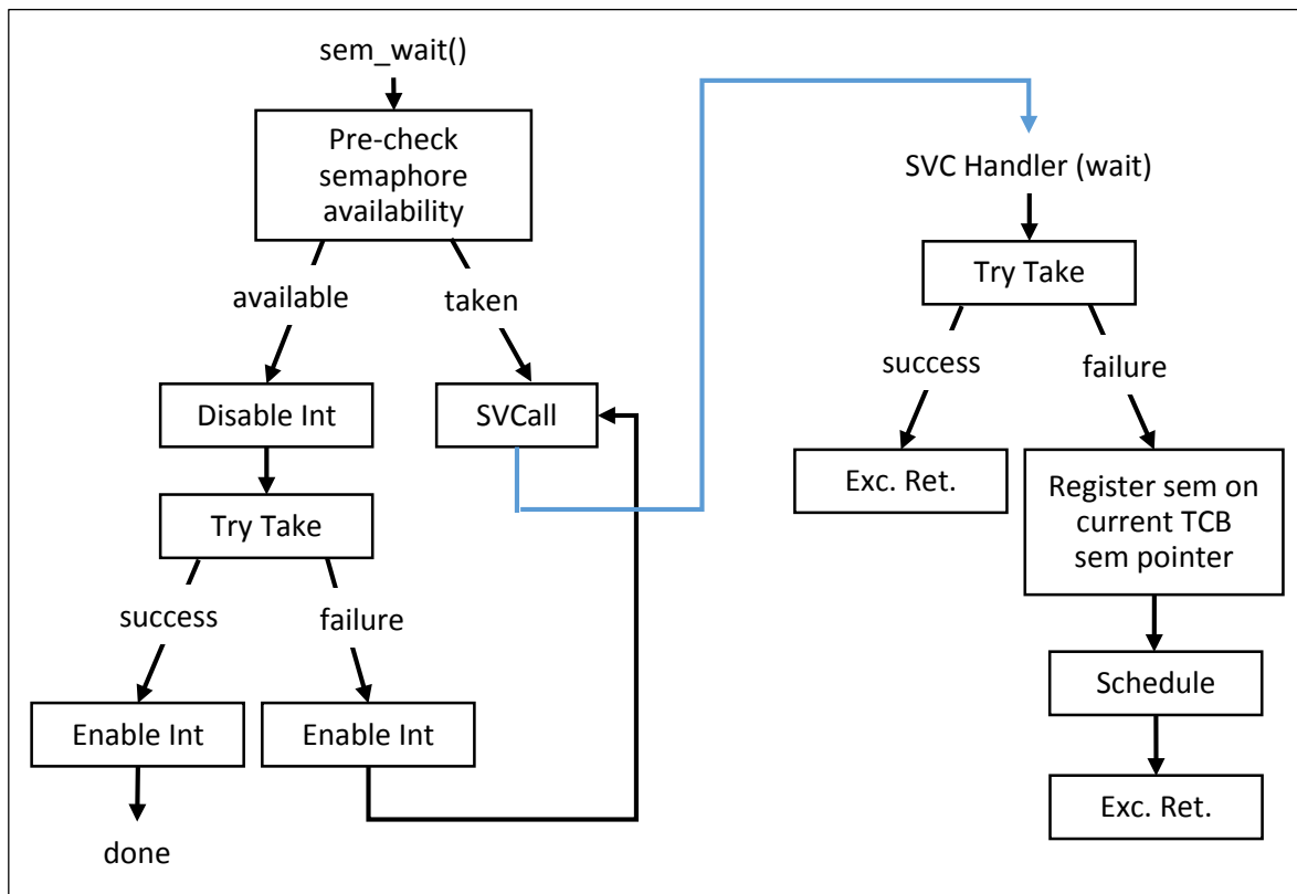
Figure 9. Semaphore Wait Operation
