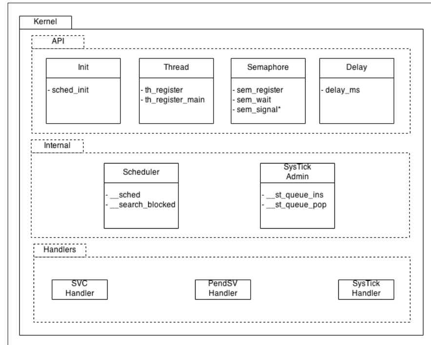
Figure 4. Kernel Detailed Architecture
