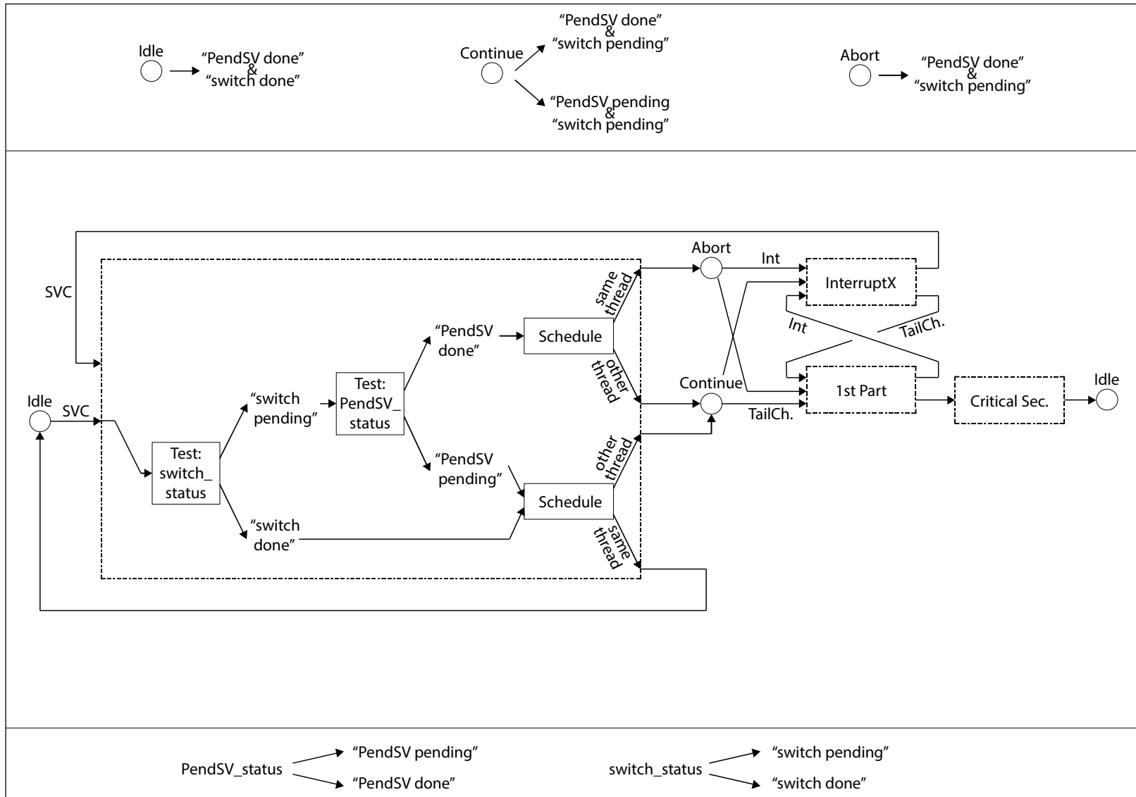
Figure 7. Context Switch State Space
