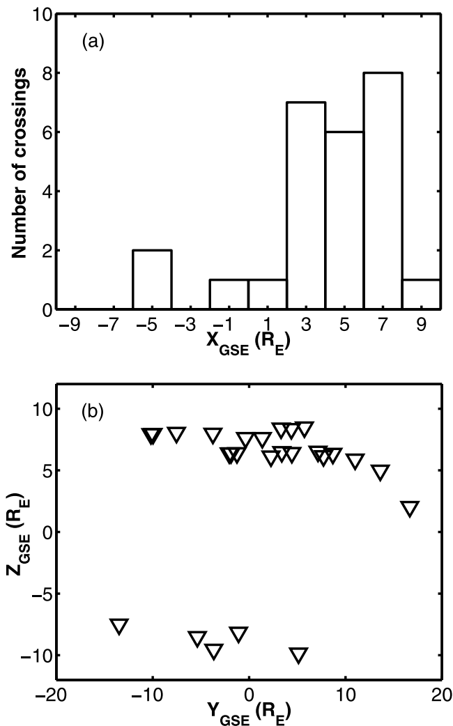
Figure 1. Overview of the locations of Cluster spacecraft, in GSE coordinates, during the magnetopause crossings used in this study. (a) The distribution of the crossings in x direction; (b) the position of the spacecraft in y-z plane.
