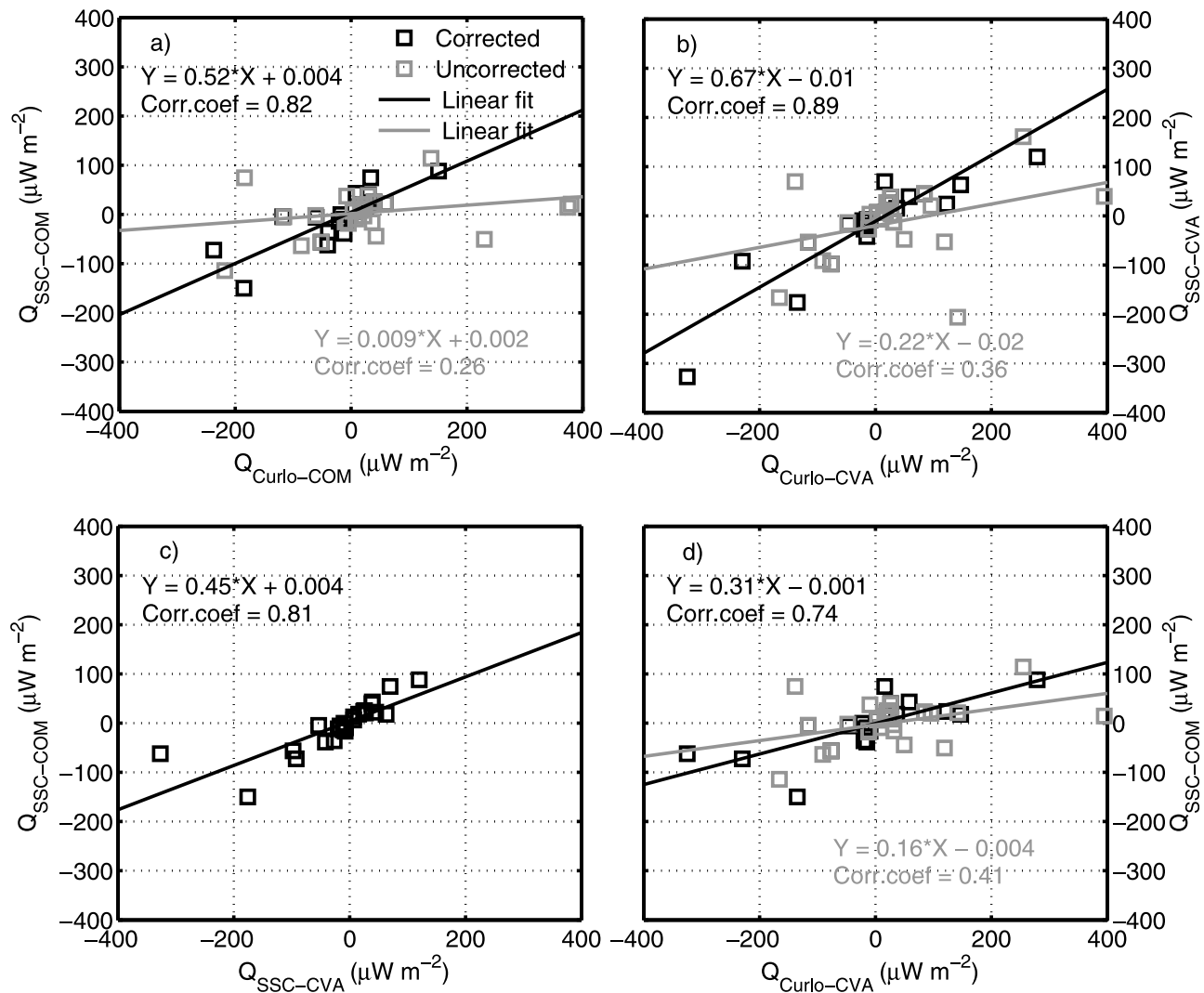
Figure 9. Demonstration of differences in energy conversion using the currents from curlometer and single-spacecraft and in multispacecraft (CVA) and single-spacecraft (COM) frames. (a) The Q using single-spacecraft and curlometer current in COM frame. (b) Q in CVA frame. (c) Q using single-spacecraft current in CVA and COM frames. (d) Q using single-spacecraft and multispacecraft methods.
