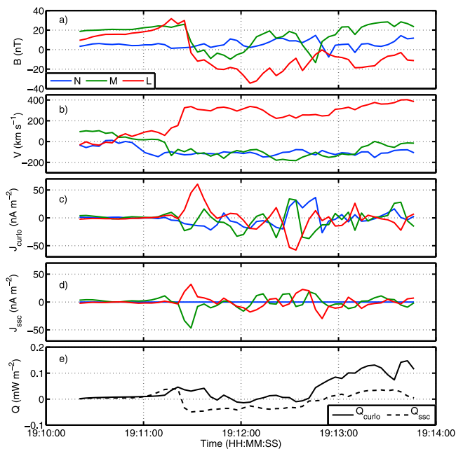
Figure 6. A magnetopause crossing on Jan 18, 2004: (a–d) magnetic field, plasma velocity, curlometer current density and the single-spacecraft current density, respectively. All the quantities are in LMN frame given by the CVA method. (e) The energy conversion estimates with curlometer current (solid line) and with single-spacecraft current (dashed line).
