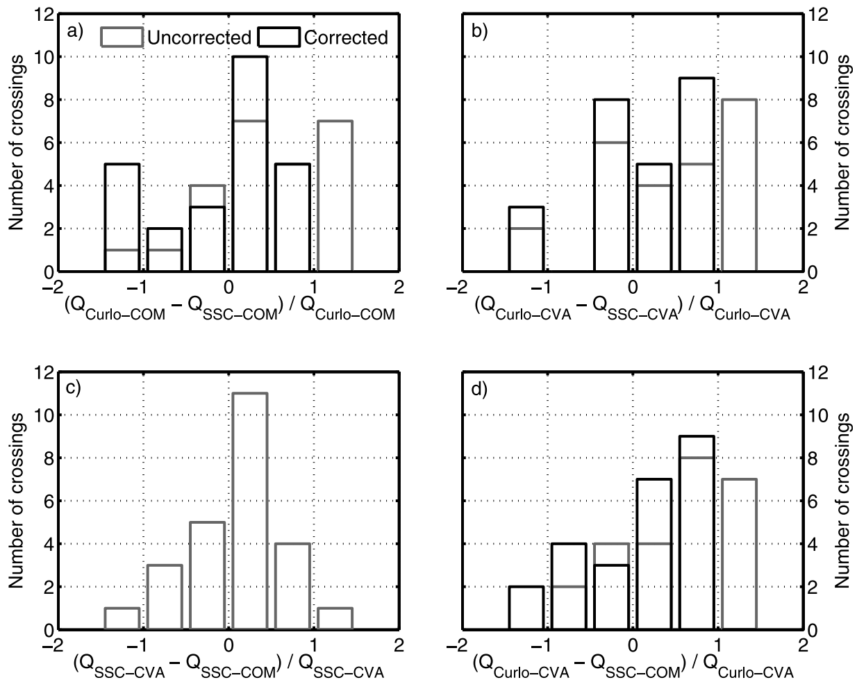
Figure 8. Statistical nature of the errors introduced by the use of single-spacecraft methods. Black (gray) lines represent energy conversion results using the corrected (uncorrected) curlometer current. (a and b) The statistics of the ambiguities introduced by the use of single-spacecraft current approximation in COM and CVA frames, respectively. (c) Statistical representation of the ambiguities introduced due to the separation between normals from the two methods; (d) the combined effect of all the ambiguities introduced by the normal, single-spacecraft current and the magnetopause velocity.
