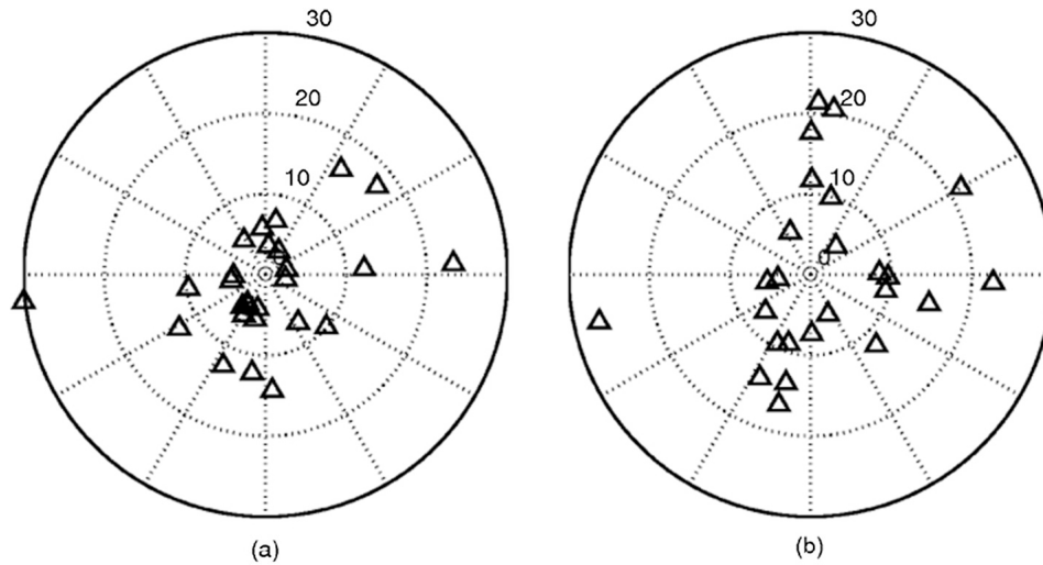
Figure 3. Polar plots showing a comparison of the orientation of the magnetopause obtained from COM and CVA methods. The position along the radial direction gives the angular separation between the normals being compared and azimuthal direction is the plane perpendicular to the reference normal given by the bull's eye. For example, at subsolar point the normal would be in the sunward direction, then the axes would roughly be the GSE y and z. In both panels, the bull's eye is the orientation provided by the CVA method and the triangles are individual magnetopause crossings. (a) Results without the use of constraints on COM and (b) results when tangential discontinuity constraint, i.e., \langle \mathbf{B} \rangle \cdot \mathbf{n} = 0 is applied on COM.
