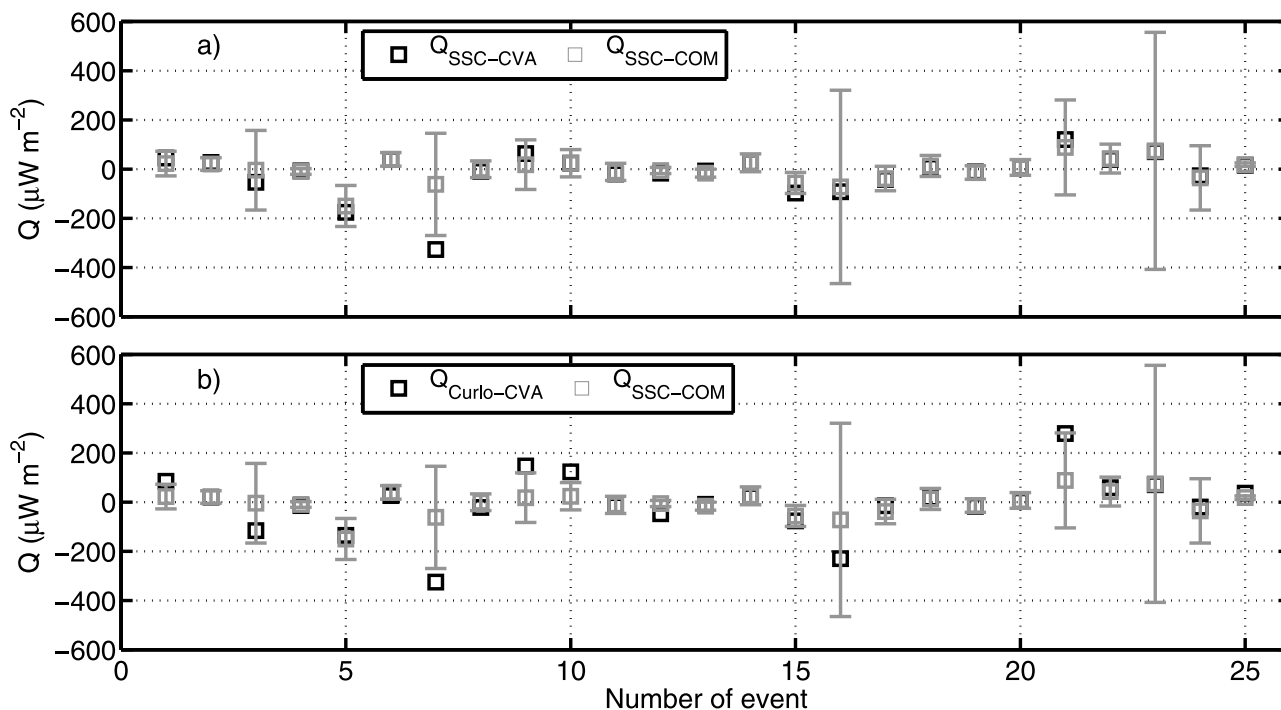
Figure 10. Demonstration of the uncertainties in the energy conversion estimates from single-spacecraft methods. (a and b) Gray squares with error bars represent the energy conversion and their associated uncertainties from single-spacecraft current in the COM frame. The black squares in Figure 10a (Figure 10b) are energy conversion estimates using single-spacecraft (curlometer) current in CVA frame.
