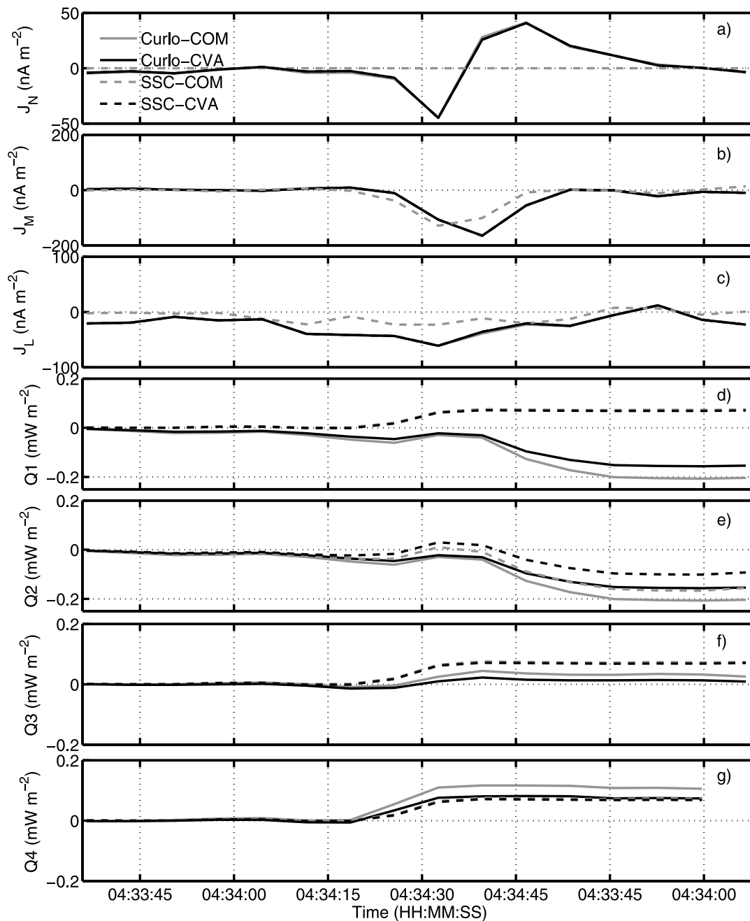
Figure 7. Current density and energy conversion during a magnetopause crossing on Apr 6, 2004, using multi and single-spacecraft methods. (a–c) The N, M and L components of magnetopause current density, respectively. The description and color coding are similar to Figures 5a–5c. (d–f) The energy conversion estimates using different values for the normal current. Figure 7d is similar to Figure 5e. In Figure 7e the solid lines use curlometer current in CVA (black) and COM (gray) frames and the dashed lines use single-spacecraft current after the normal current being replaced by the normal current from curlometer. In Figure 7f the dashed lines use the single-spacecraft current whereas the solid lines use the current from curlometer with zero normal current. (g) The energy conversion similar to Figure 7f but the curlometer current is moved backwards in time to match the peak of the major component of current (M) from the single-spacecraft method.
