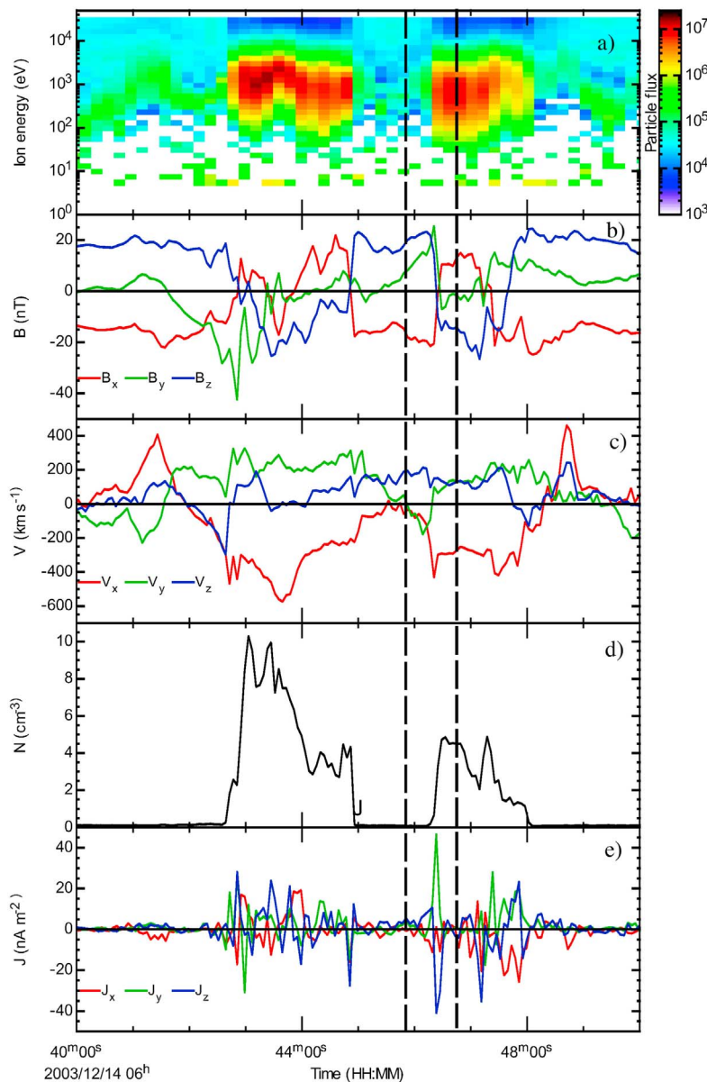
Figure 2. Cluster spacecraft 1 measurements on 14 December, 2003 on an outbound crossing. Shown here are (a) omnidirectional ion energy spectrogram, (b) magnetic field, (c) ion bulk velocity, (d) ion density, and (e) current density estimated using the curlometer technique. The two vertical dashed lines indicate the time period of the magnetopause crossing examined in this paper.
