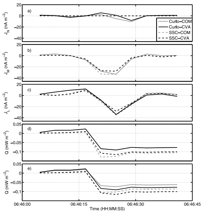
Figure 5. Estimated current density and energy conversion during a magnetopause crossing on Dec 14, 2003 using multi and single-spacecraft methods. The black (gray) curves are in boundary normal frame determined by CVA (COM) method, whereas the solid (dashed) lines are currents estimated using curlometer (single-spacecraft) method. (a–c) The N, M and L components of the current density, respectively. (d and e) The estimated energy conversion using curlometer (solid lines) and single-spacecraft currents (dashed lines) in CVA (black lines) and COM frames (gray lines). All the curves represented in Figure 5d use same magnetopause velocity (from CVA, 135.8 km/s) in energy conversion estimation whereas the black (gray) lines in Figure 5e use the magnetopause velocity given by CVA (COM) methods.
