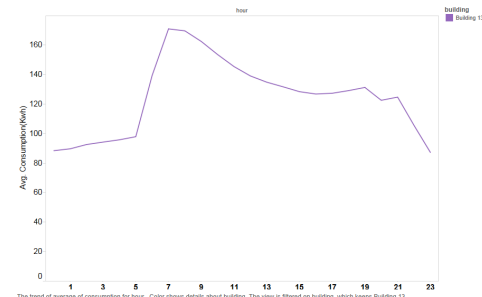
The trend of average of consumption for hour. Color shows details about building. The view is filtered on building, which keeps Building 13.
