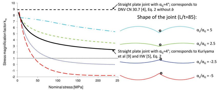
Figure 10: Stress magnification factor k_m as a function of the applied load for different specimen shapes [P1].
