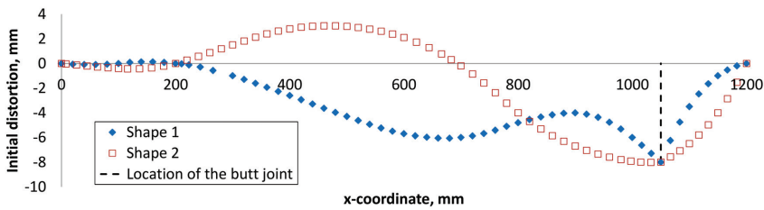
Figure 17: Initial distortion in the longitudinal, i.e., the stiffener direction, in the middle of the plate field [P3].
