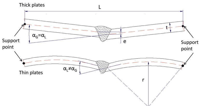
Figure 5: Definition of the initial distortion in the thick (top) and thin (bottom) specimens [P1].
