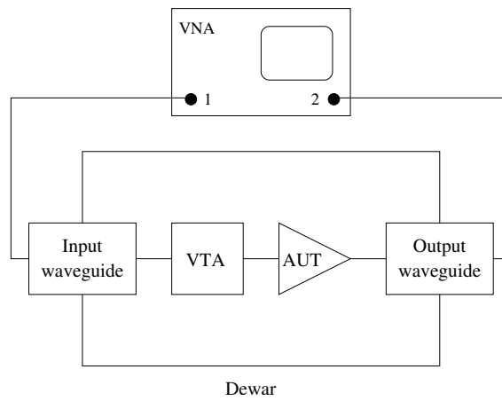
Figure 37: Cryogenic measurement setup for obtaining the gain of the amplifier.
