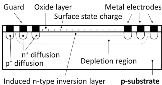
Figure 4. Simplified cross-section of the developed induced junction photodiodes (not to scale). For reflectance loss calculations, also a nanometer range mixture layer of \text{SiO}_2 and Si at the oxide - silicon interface and a top layer of ice-like water on \text{SiO}_2 are used, but not depicted here. (Publication IV).
