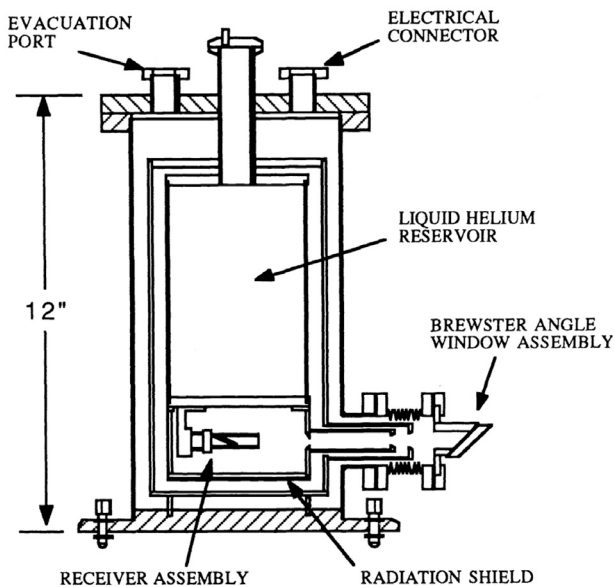
Figure 2. Example of a liquid helium cooled cryogenic radiometer. Figure from [44].
