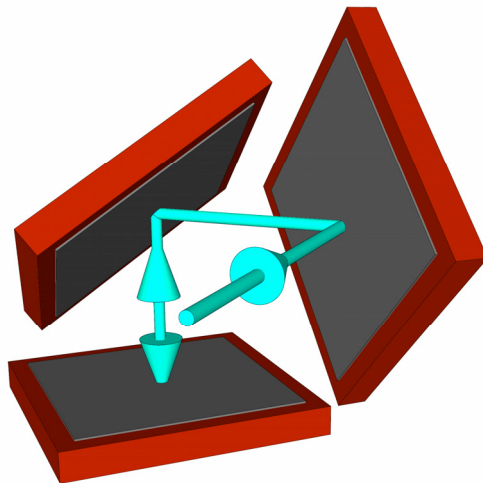
Figure 1. Trap detector consisting of three photodiodes. Five reflections and varying planes of incidence make this type of detector polarization independent.
