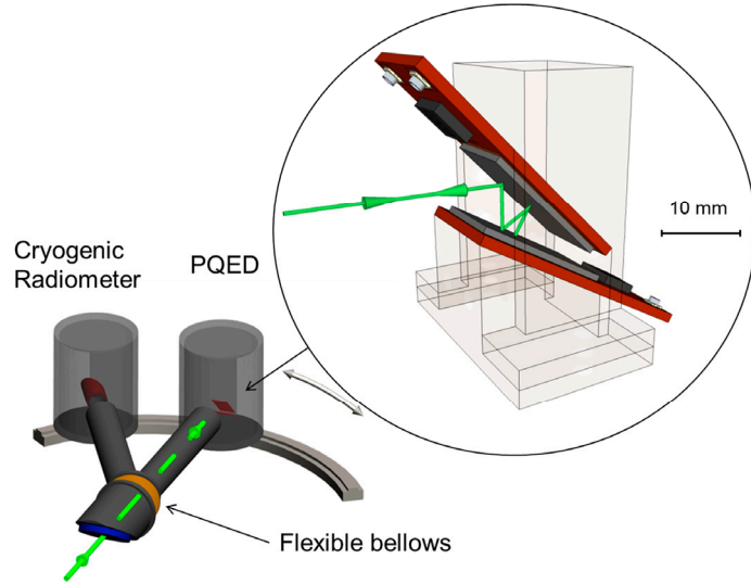
Figure 12. PQED responsivity measurement setup at PTB showing the cryogenic radiometer and PQED on an arc-shaped rail behind the joint Brewster window. The magnified section of PQED shows the photodiode arrangement inside a copper holder (semi-transparent area) for efficient heat transfer from the cryostat cold finger to the photodiodes.
