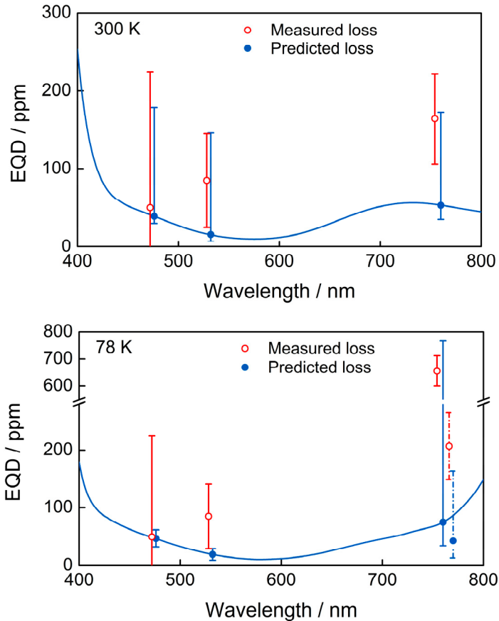
Figure 13. Measured and predicted external quantum deficiency (EQD) at room temperature and at liquid nitrogen temperature with reverse bias voltage of 5V. Measurements were made at the wavelengths of 476 nm, 532 nm and 760 nm. The uncertainty bars show expanded uncertainty in the confidence level of 95 %. The points with dashed uncertainty bars indicate predicted and measured EQD and their uncertainties at the reverse bias voltage of 20V.
