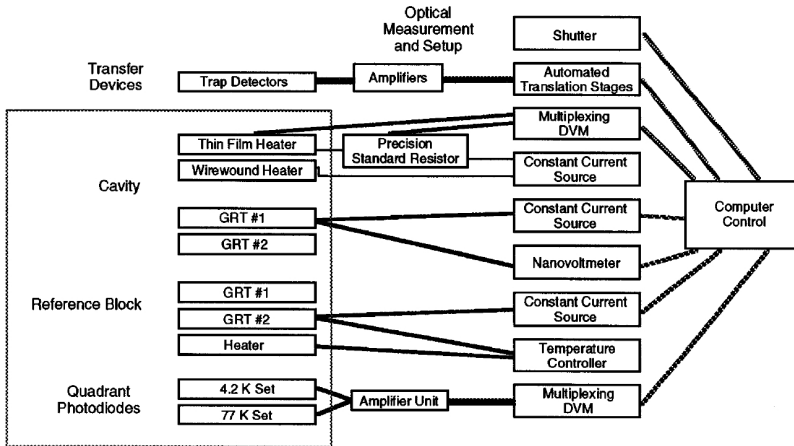
Figure 3. Example diagram of the CR measurement instrumentation used in NIST. The elements surrounded by the box are inside the CR Dewar. Most of the controlling apparatus is required for operating the CR. Such complex instrumentation is typical for all CR systems. See also Figure 14 showing the simple instrumentation setup if the primary standard is realized with a solid state detector. Figure taken from [47]
