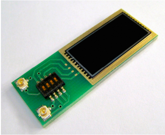
Figure 8. Processed PQED photodiode mounted on the PCB board. Photocurrent is registered using the U.FL connectors. Same contacts are used to apply the bias voltage. The small 4-channel switch routes signals between contacts and allows using different operational modes, when necessary. (Publication IV).
