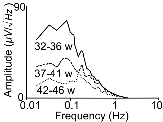
Figure 3. Changes in the lowest frequencies of EEG due to maturation. Note logarithmic frequency scale. EEG spectra are dominated by frequencies below 1 Hz, especially in the preterm infants (conceptional age 32-36 weeks). Adapted from Vanhatalo et al. (2005).
