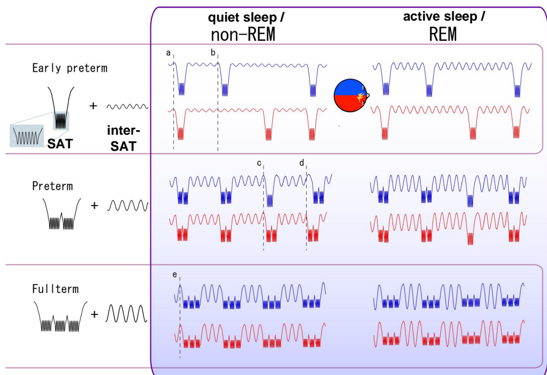
Figure 2. Development of SAT events and ongoing oscillatory activity during inter-SATs in preterm babies. Adapted from (Vanhatalo, Kaila 2006).
