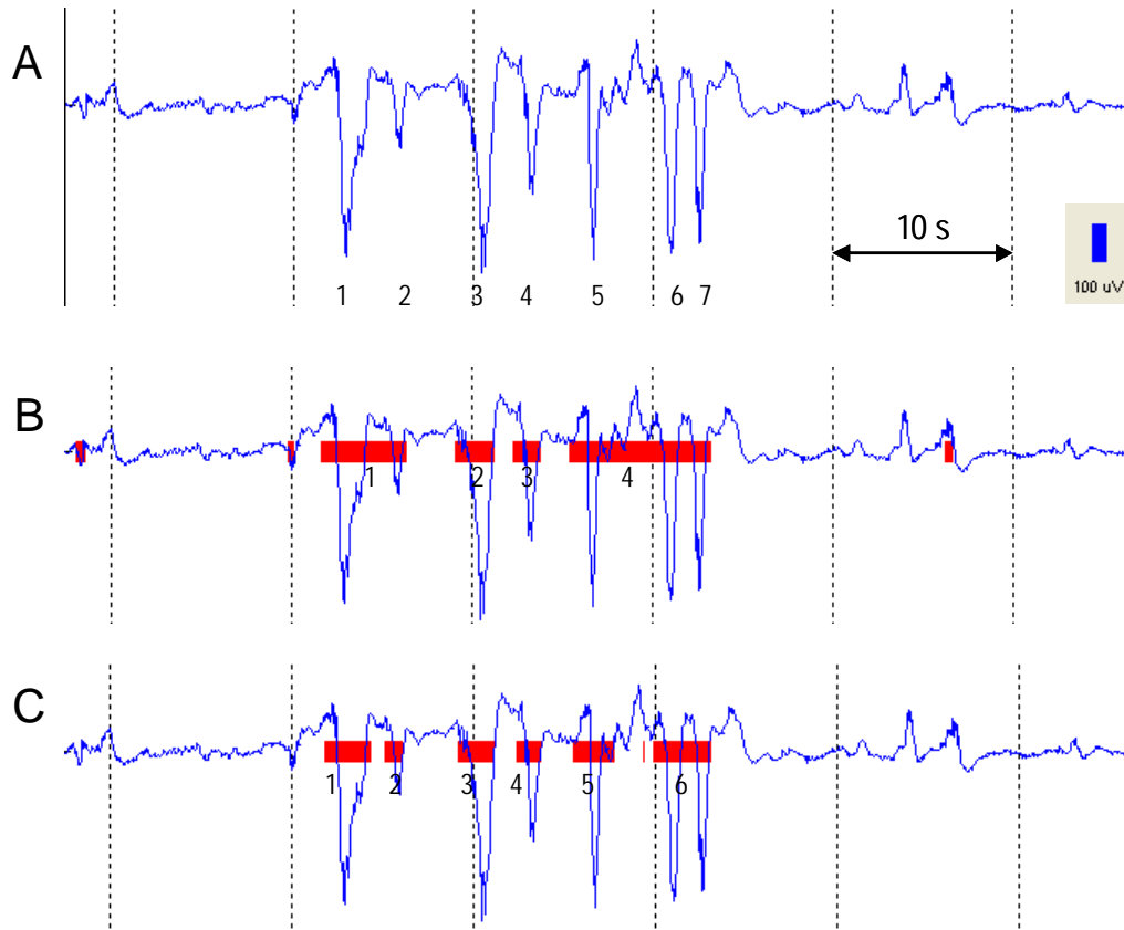
Figure 7: Example of automated detection of SATs with different thresholds. Threshold has a strong effect on SAT number and mean SAT duration but a smaller effect on SAT%. A: EEG with 7 visually clear SATs in the middle. B: Result of automated SAT detection algorithm (unpublished). Using a low threshold, some of the SATs are merged together in the automated detection. Four SAT periods lasting at least one second are detected. C: Higher threshold leads to separation of SATs in the automated detection. Six SAT periods are detected.
