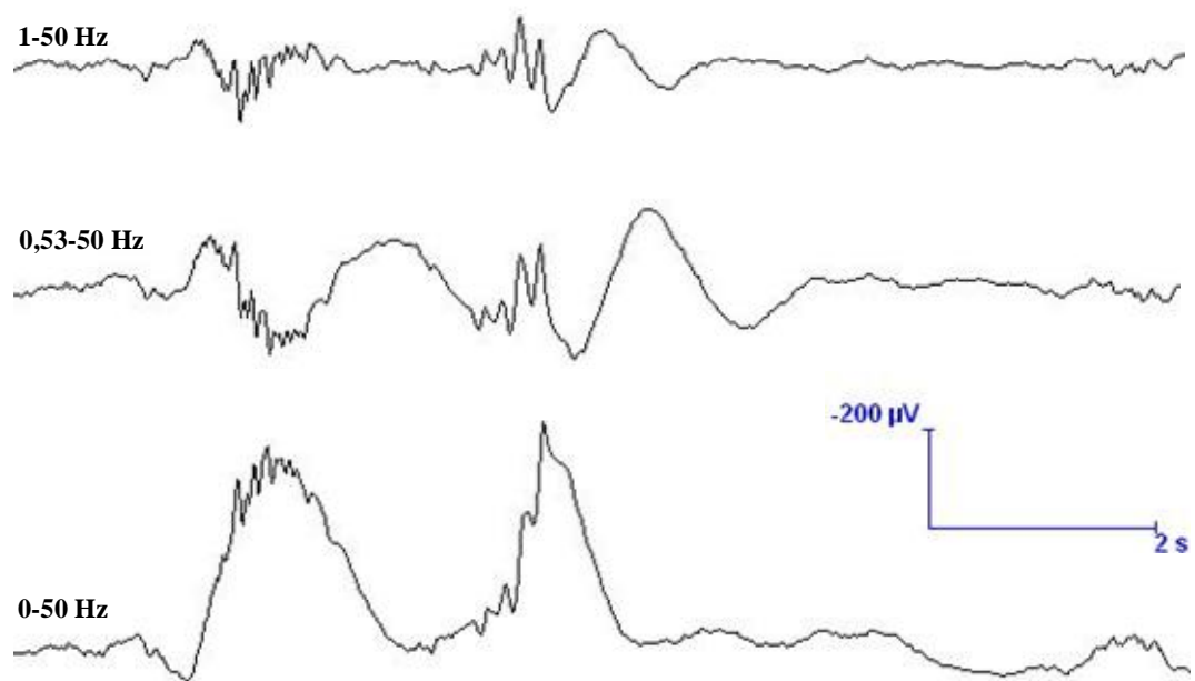
Figure 1. Preterm EEG with two SATs. EEG shown both without filtering (bottom) and with some conventional filter settings. Conventional high pass filtering heavily distorts the appearance of the SATs. (Palmu 2008)
