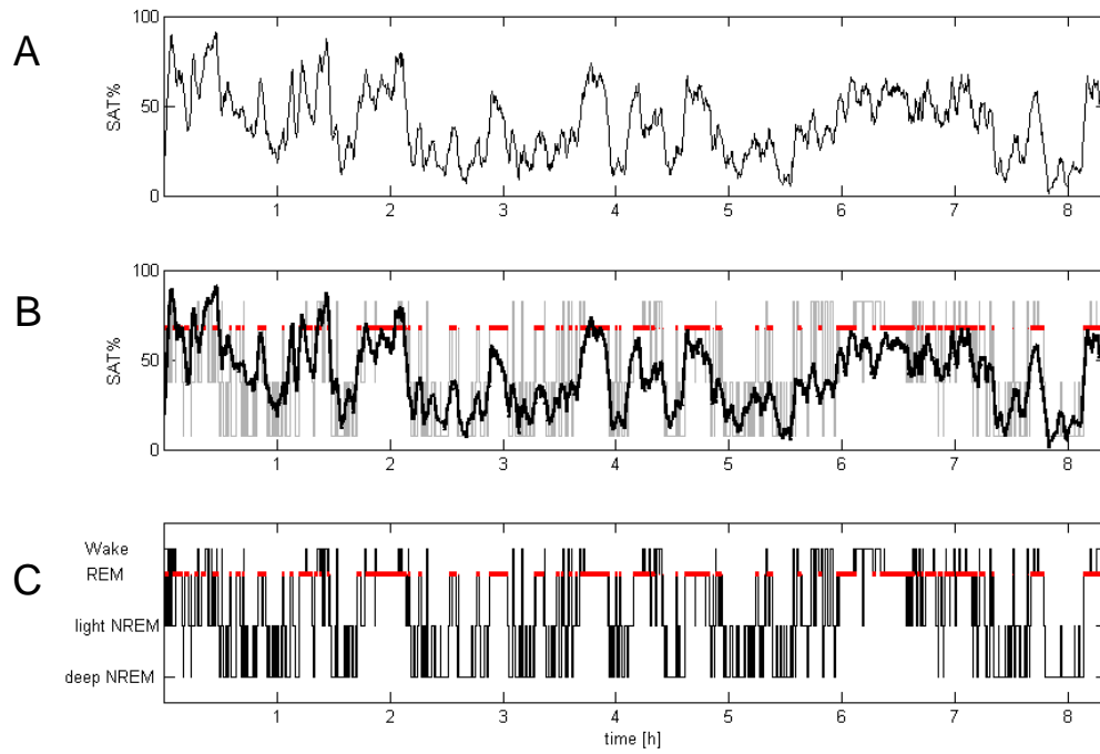
Figure 8: A. Example of SAT% fluctuation with time in an infant at conceptional age of 26 weeks. SAT% was calculated in 3 min epochs. C: Manual scoring of sleep stages. B: SAT% and scoring results overlaid. Note how SAT% increases during REM epochs and is very low during deep NREM epochs. The infant in this example is quite sick and demands mechanical ventilation. Sleep is fractionary with many transitions between sleep stages. Nevertheless several sleep cycles can be observed with cycle length of approximately half an hour.
