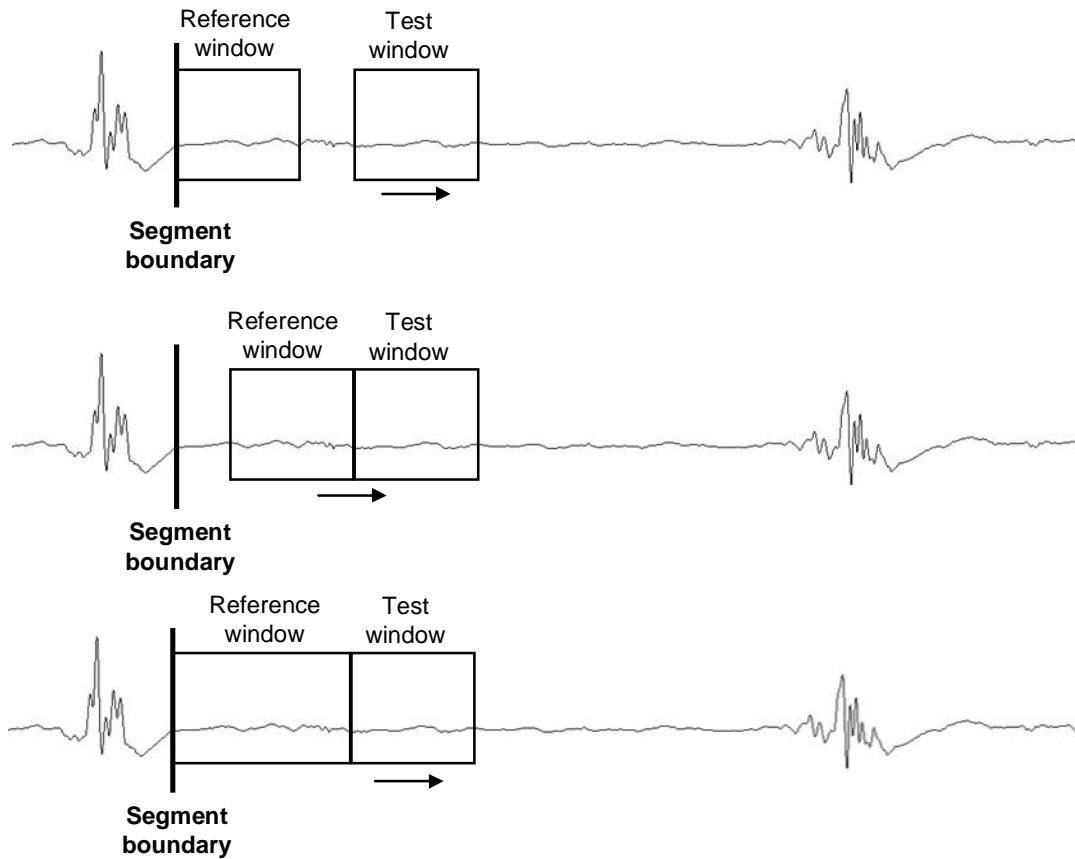
Figure 6: Different definitions of reference and test windows. Reproduced based on (Wong 2008)
