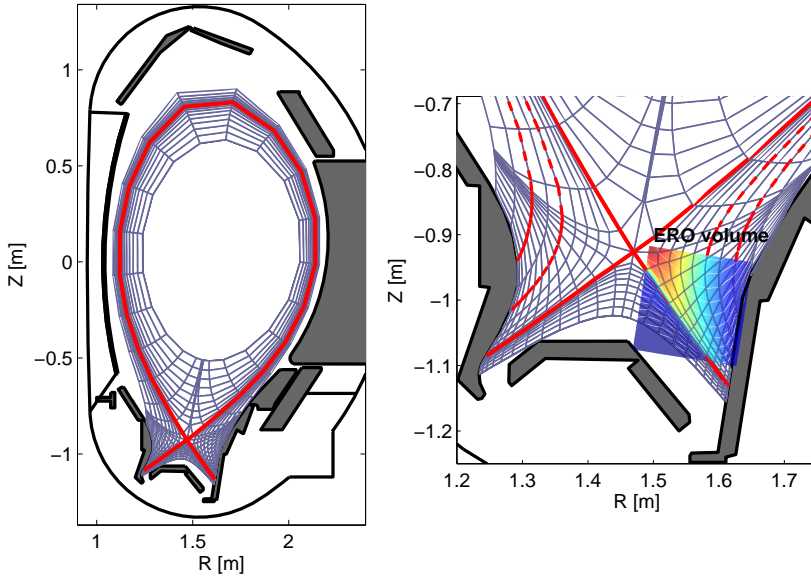
Figure 4.1: SOLPS5.0 (left) and ERO (right) simulation regions.
