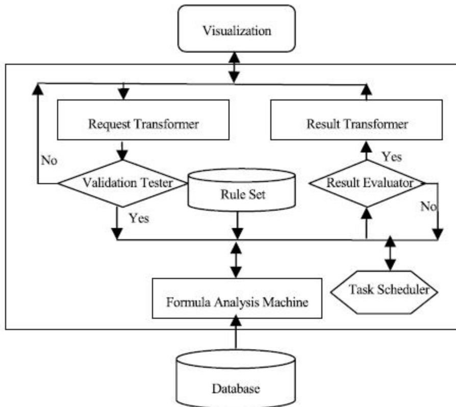
Figure 24: Workflow of KISTCM (Qiao et al., 2008)
