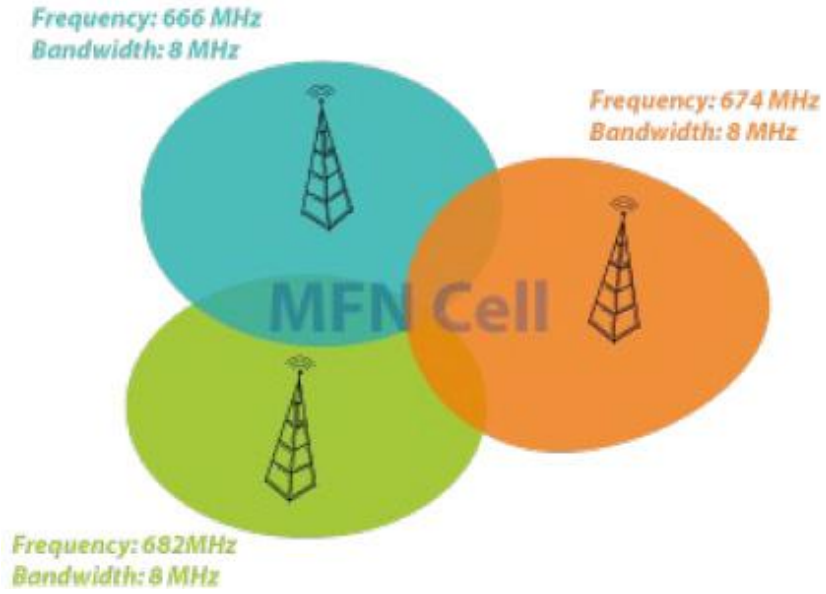
Figure 2.1 MFN topology
