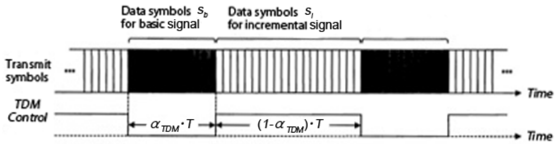
Figure 3.3 TDM scheme
