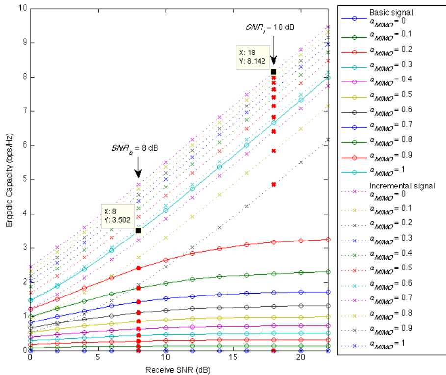
Figure 5.10 Hierarchical MIMO ergodic capacity for basic signal and incremental signals (with correlation)
