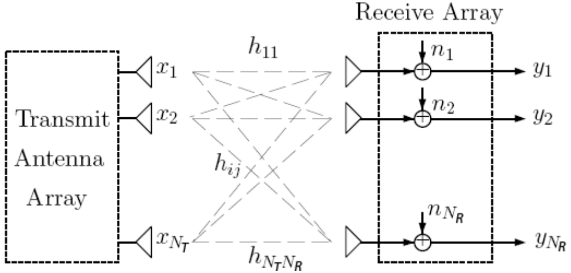
Figure 2.9 MIMO system model
