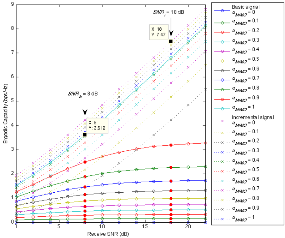
Figure 5.8 Hierarchical 2 \times 2 MIMO ergodic capacities for basic and incremental signals (no correlation)
