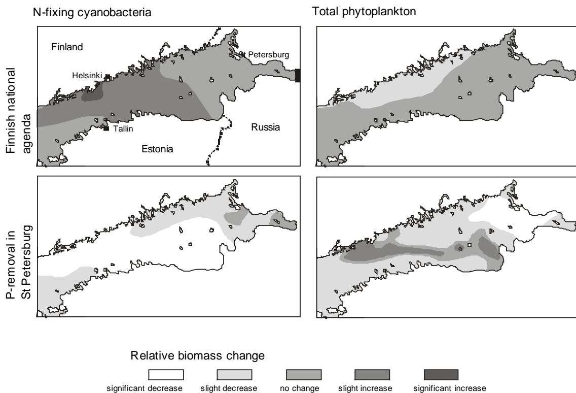
Figure 7. The effects of load reductions on the average total and cyanobacteria biomass (VI).
