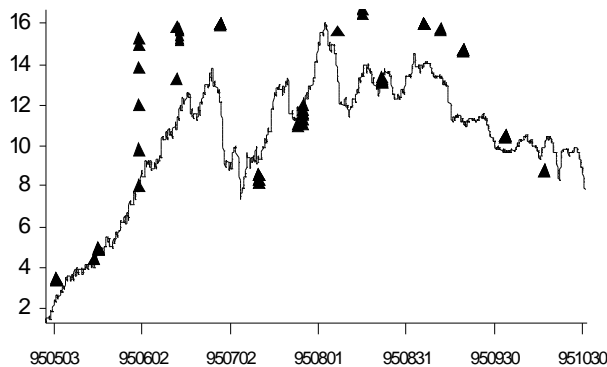
Figure 3. Simulated and measured salinity (ppm) and temperature ( ^{\circ}\text{C} ) from point HKVV Gulf of Finland (I).
