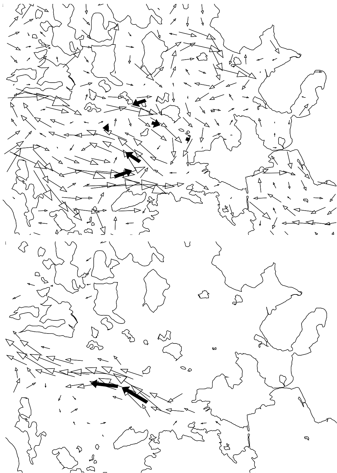
Figure 4. Calculated flow field compared to the results of regression model. Upper field is from layer 0-2 m and downer from 6-8 m depth. Wind is 5 m/s from west. (II)
